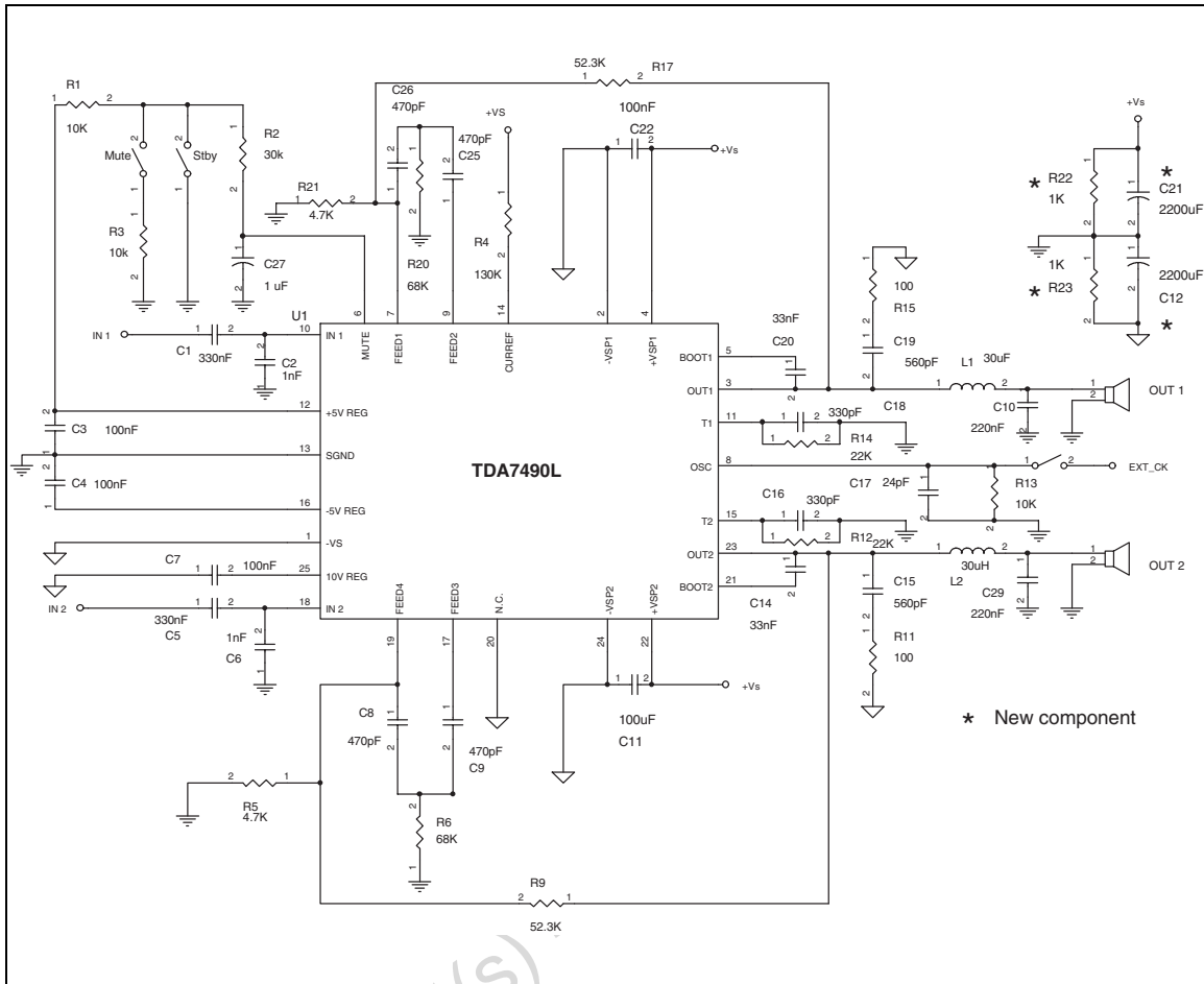
Figure 4. Application in Supply Voltage
