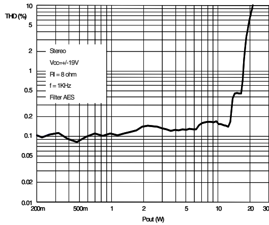
Figure 8. Distortion vs. Output Power
