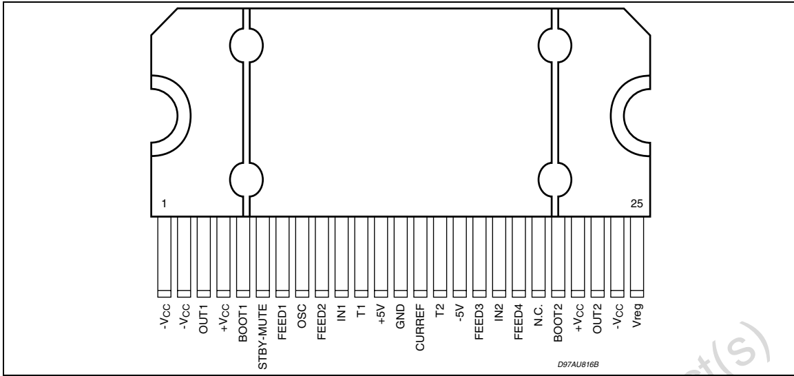
Figure 5. Pin Connection
