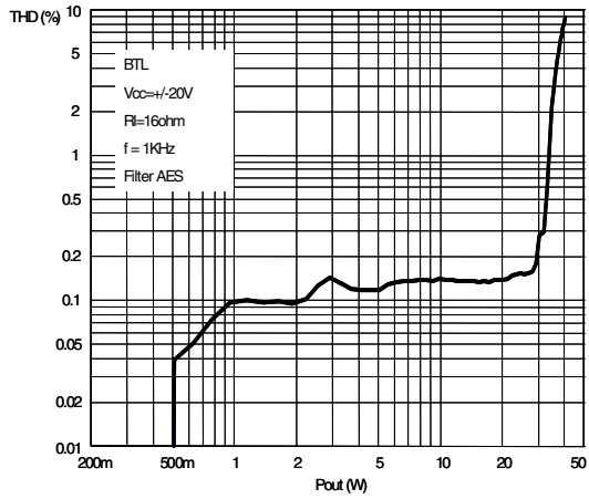
Figure 13. Distortion vs. Output Power in BTL
