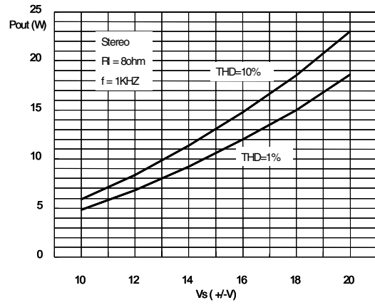
Figure 14. Pout vs Supply Voltage
