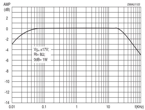
Figure 10. Frequency Response
