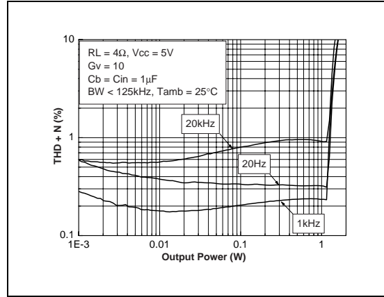
Fig. 28 : THD + N vs Output Power
