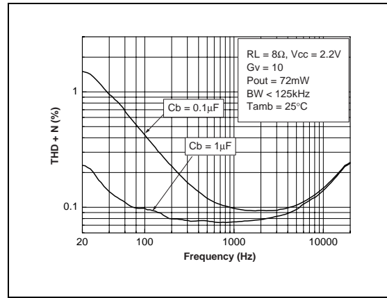
Fig. 82 : THD + N vs Frequency
