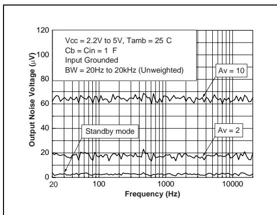
Fig. 101 : V_{out1}+V_{out2} Unweighted Noise Floor
