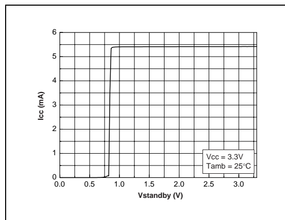
Fig. 96 : Current Consumption vs Standby Voltage @ Vcc = 3.3V
