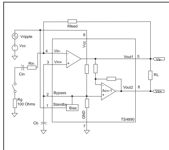
Fig. 108 : PSRR measurement schematic
