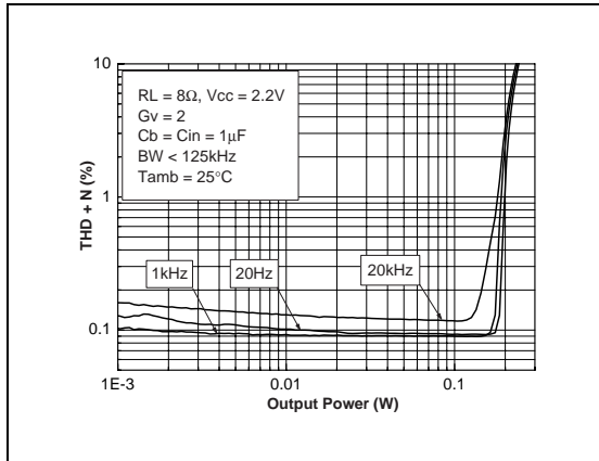
Fig. 41 : THD + N vs Output Power
