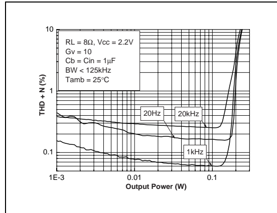
Fig. 42 : THD + N vs Output Power
