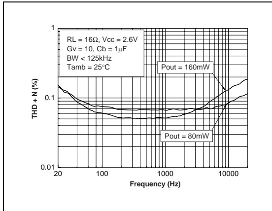
Fig. 87 : THD + N vs Frequency
