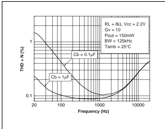
Fig. 81 : THD + N vs Frequency
