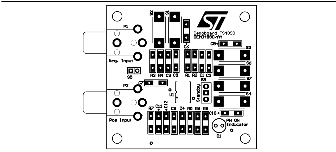
Fig. 104 : SO8 & MiniSO8 Demoboard Components Side
