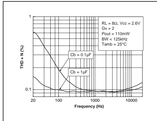
Fig. 76 : THD + N vs Frequency
