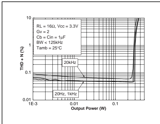
Fig. 53 : THD + N vs Output Power
