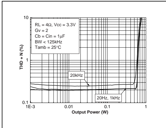
Fig. 29 : THD + N vs Output Power
