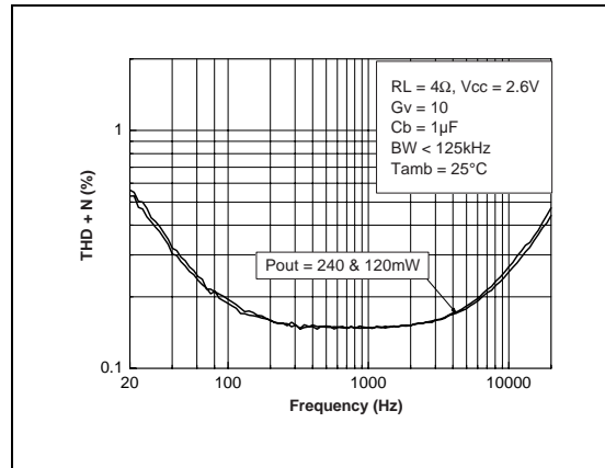
Fig. 64 : THD + N vs Frequency
