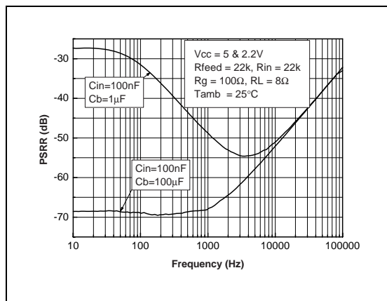
Fig. 107 : PSRR changes with Cb
