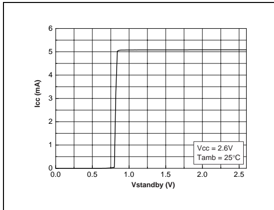
Fig. 97 : Current Consumption vs Standby Voltage @ V_{cc} = 2.6V
