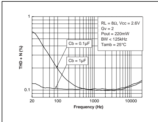
Fig. 75 : THD + N vs Frequency
