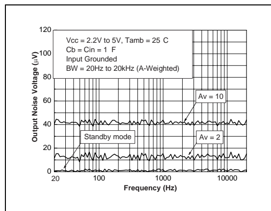
Fig. 102 : V_{out1}+V_{out2} A-weighted Noise Floor
