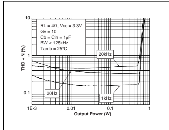
Fig. 30 : THD + N vs Output Power
