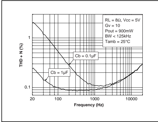
Fig. 69 : THD + N vs Frequency
