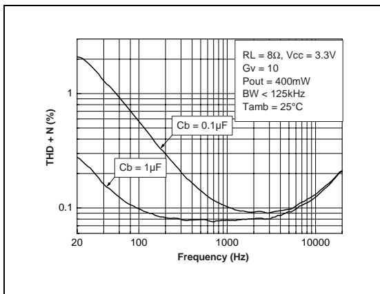
Fig. 71 : THD + N vs Frequency
