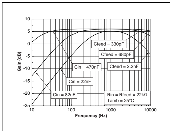
Fig. 93 : Frequency Response Gain vs Cin, & Cfeed
