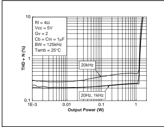
Fig. 27 : THD + N vs Output Power
