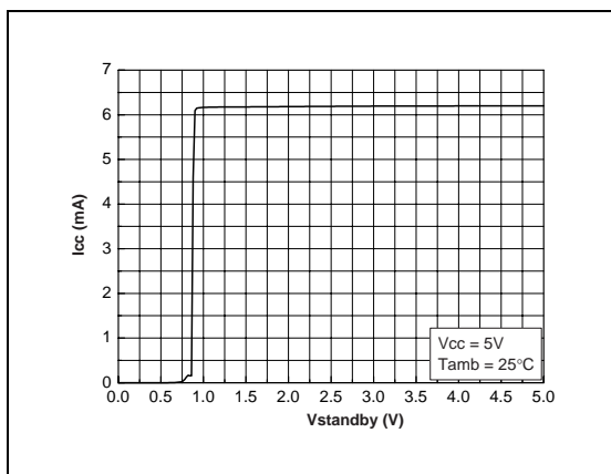
Fig. 95 : Current Consumption vs Standby Voltage @ Vcc = 5V
