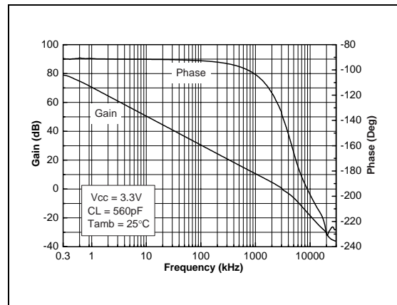
Fig. 10 : Open Loop Frequency Response
