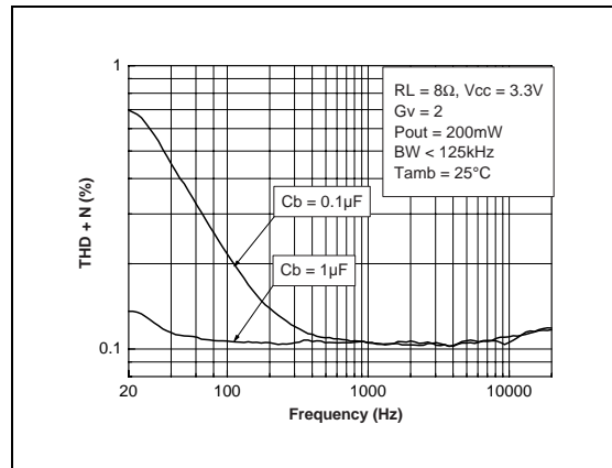
Fig. 72 : THD + N vs Frequency
