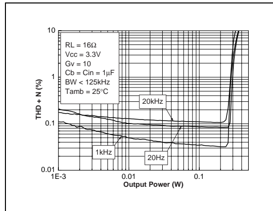
Fig. 54 : THD + N vs Output Power
