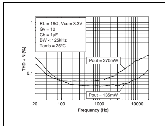
Fig. 84 : THD + N vs Frequency
