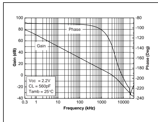
Fig. 12 : Open Loop Frequency Response
