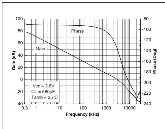
Fig. 11 : Open Loop Frequency Response
