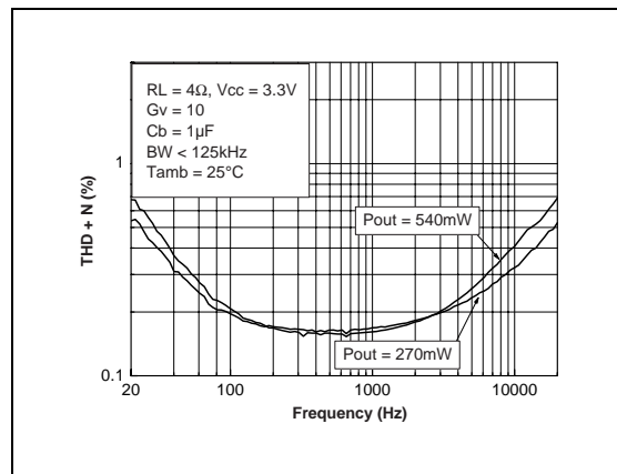
Fig. 60 : THD + N vs Frequency
