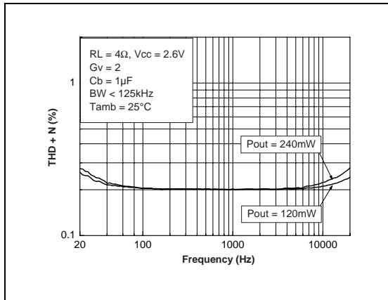
Fig. 63 : THD + N vs Frequency
