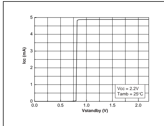
Fig. 98 : Current Consumption vs Standby Voltage @ V_{cc} = 2.2V
