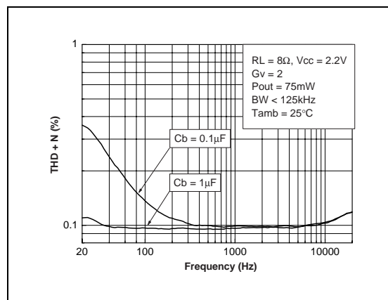
Fig. 78 : THD + N vs Frequency
