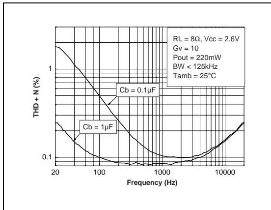
Fig. 77 : THD + N vs Frequency
