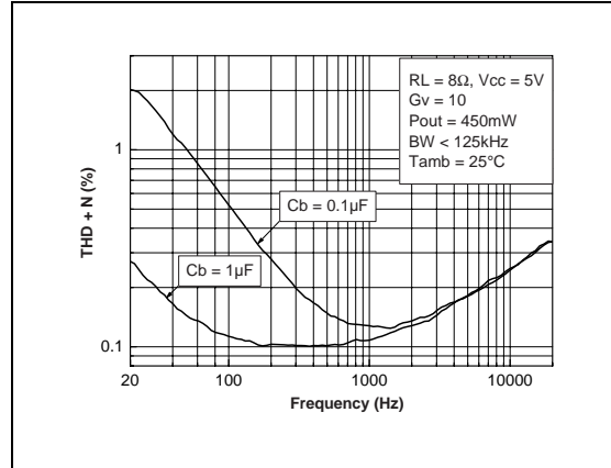
Fig. 70 : THD + N vs Frequency
