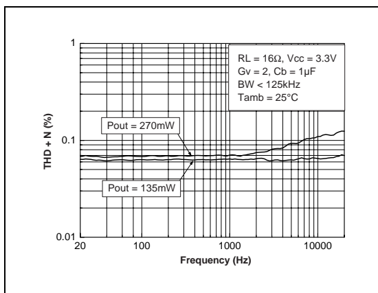
Fig. 83 : THD + N vs Frequency
