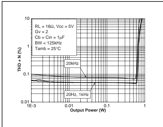
Fig. 51 : THD + N vs Output Power
