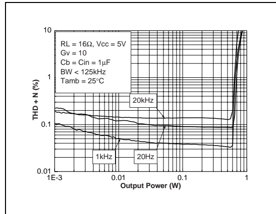
Fig. 52 : THD + N vs Output Power
