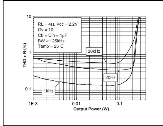
Fig. 34 : THD + N vs Output Power
