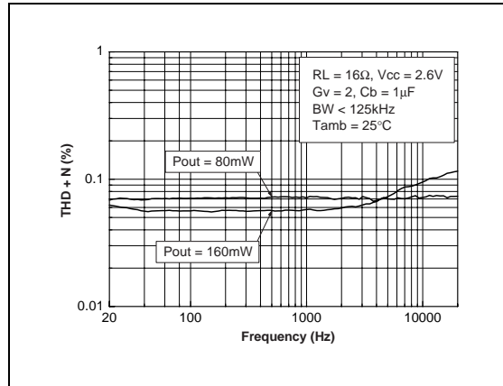
Fig. 88 : THD + N vs Frequency
