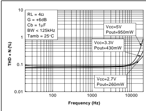
Figure 14. THD+N vs. frequency
