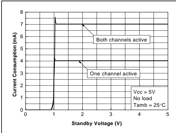
Figure 50. Current consumption vs. standby voltage
