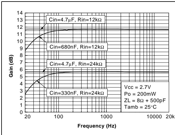
Figure 56. Frequency response
