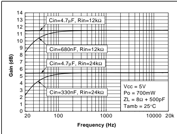
Figure 54. Frequency response
