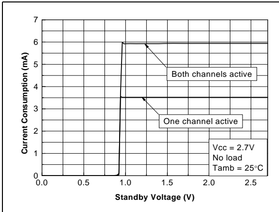
Figure 52. Current consumption vs. standby voltage
