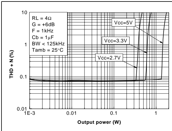
Figure 4. THD+N vs. output power
