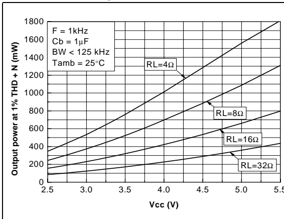
Figure 58. Output power vs. power supply voltage
