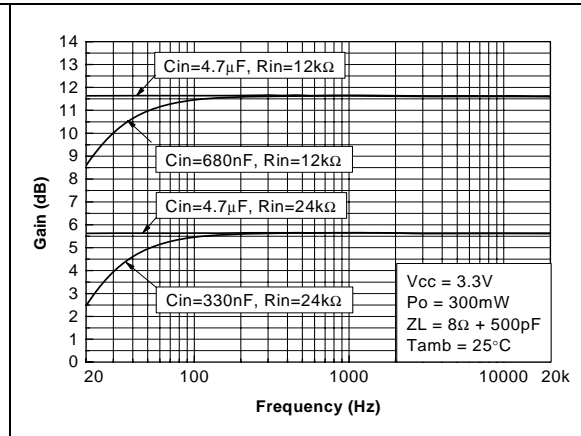
Figure 55. Frequency response
