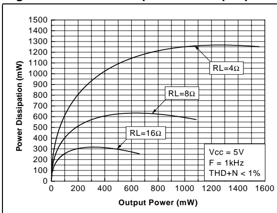
Figure 60. Power dissipation vs. output power
