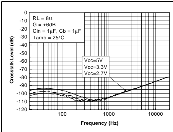
Figure 38. Crosstalk vs. frequency
