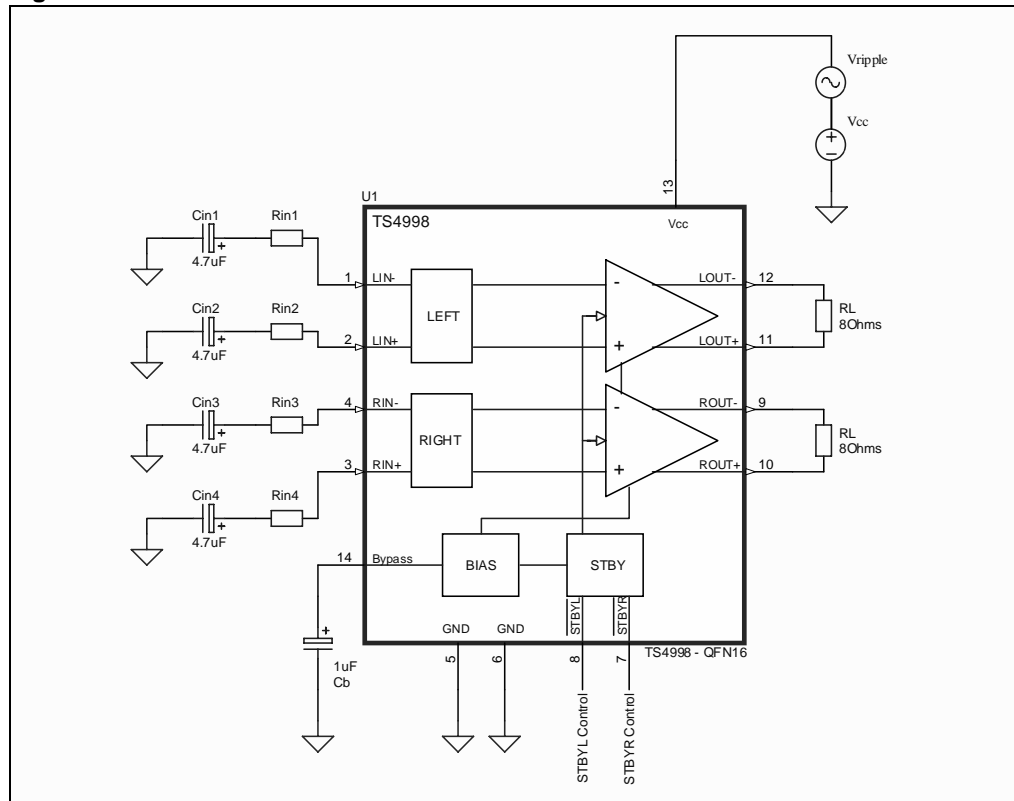
Figure 68. PSRR measurement
