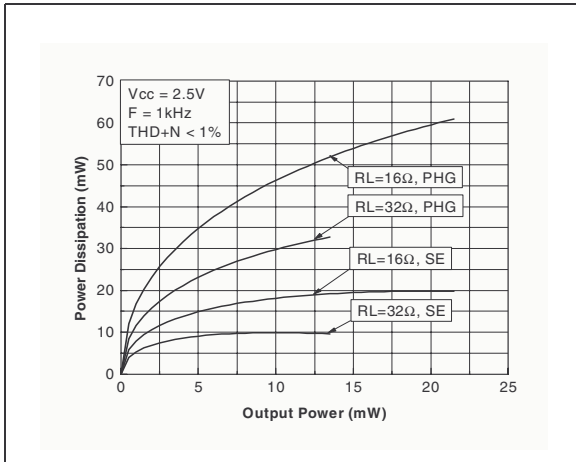
Figure 55. Power dissipation vs. output power (one channel)
