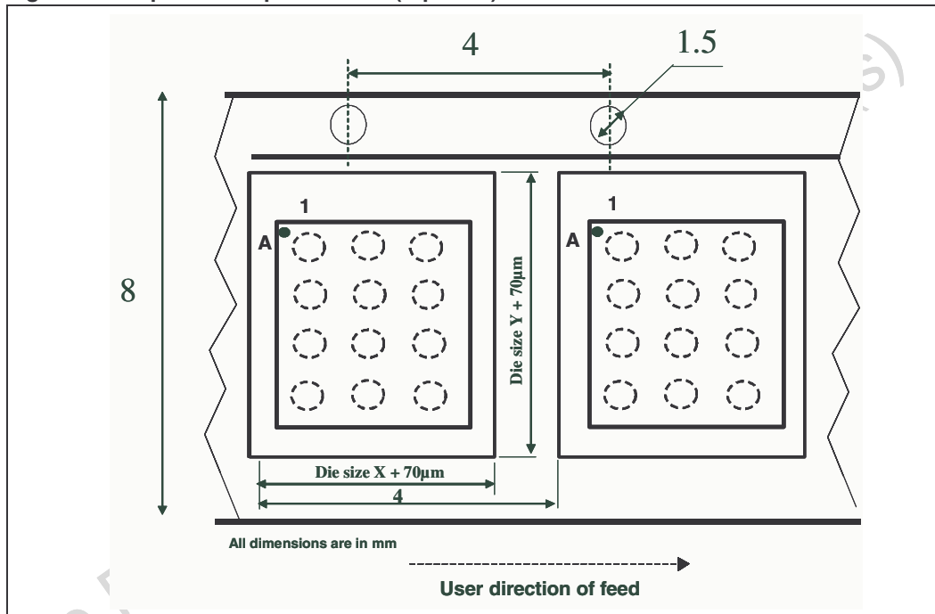
Figure 72. Tape & reel specification (top view)
