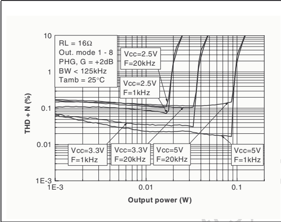
Figure 11. THD+N vs. output power
