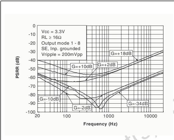
Figure 33. PSSR vs. frequency
