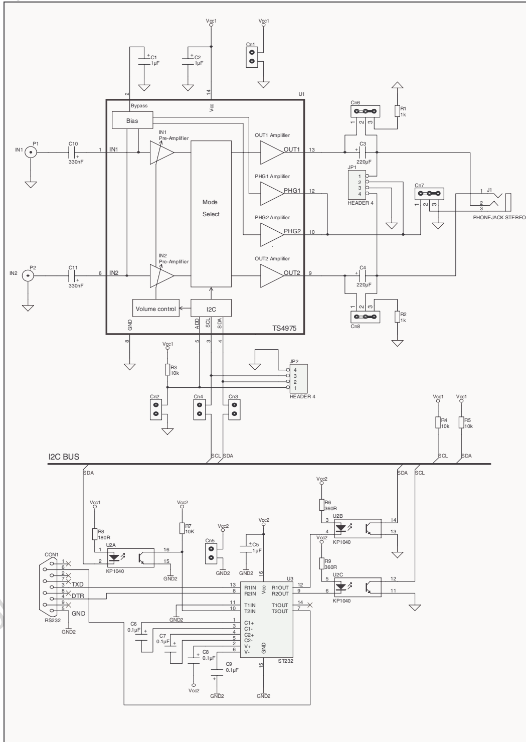
Figure 67. Demoboard schematic
