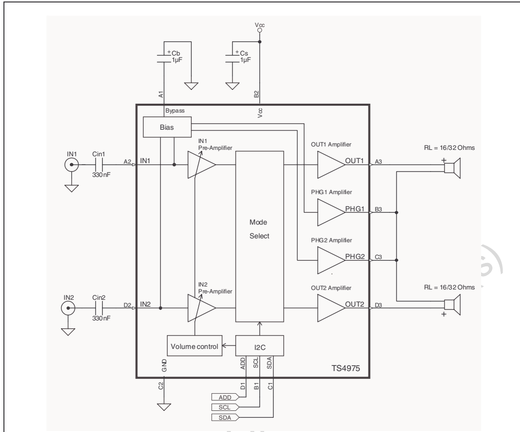
Figure 2. Phantom ground output configuration
