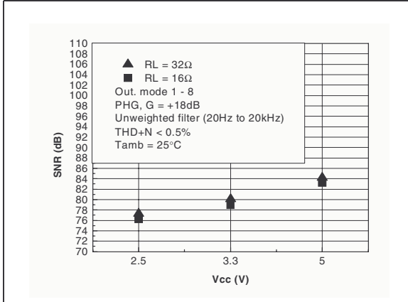
Figure 49. SNR vs. power supply voltage
