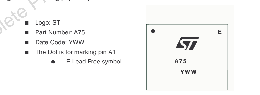
Figure 70. Marking (top view)
