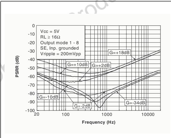
Figure 35. PSSR vs. frequency
