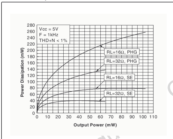
Figure 57. Power dissipation vs. output power (one channel)
