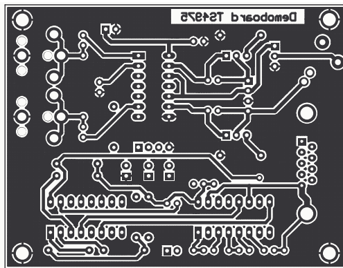
Figure 64. Bottom layer
