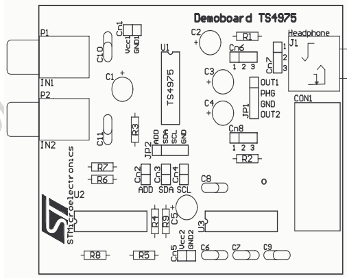
Figure 66. Component location
