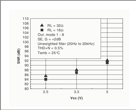
Figure 43. SNR vs. power supply voltage
