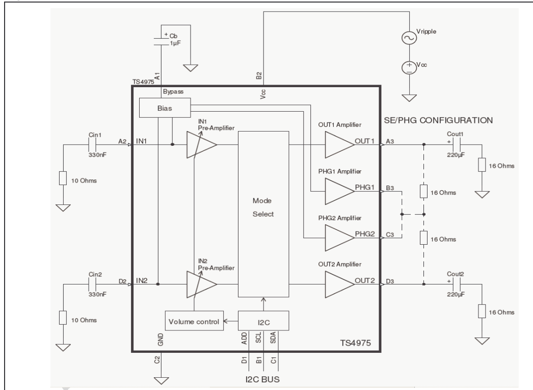
Figure 62. PSRR measurement schematic
