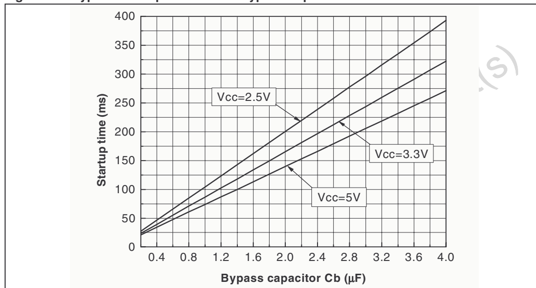
Figure 63. Typical startup time versus bypass capacitance
