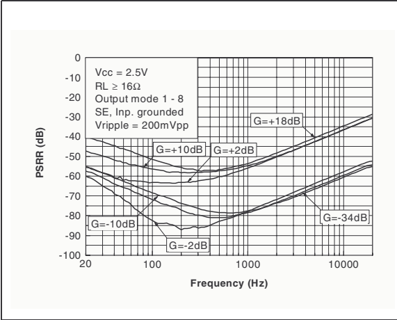
Figure 31. PSSR vs. frequency
