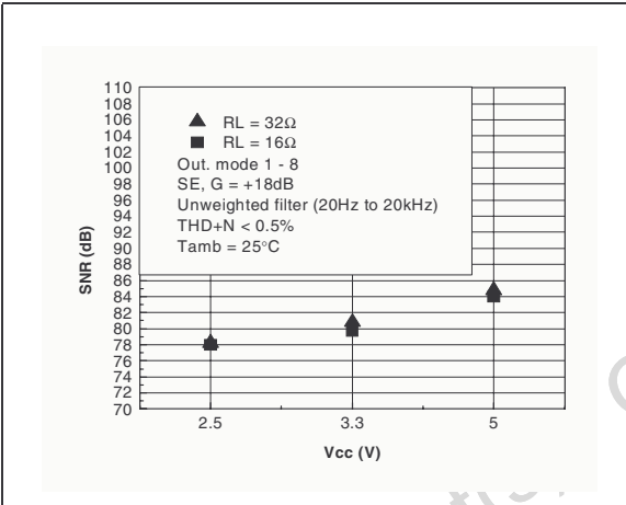
Figure 47. SNR vs. power supply voltage
