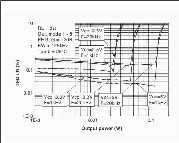
Figure 9. THD+N vs. output power
