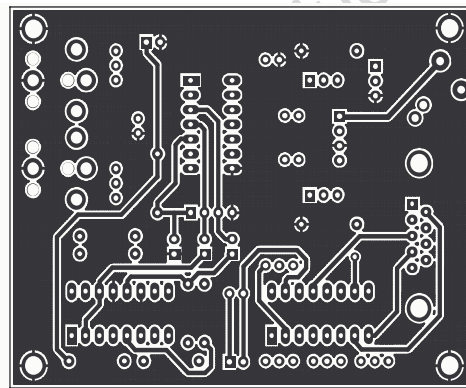
Figure 65. Top layer
