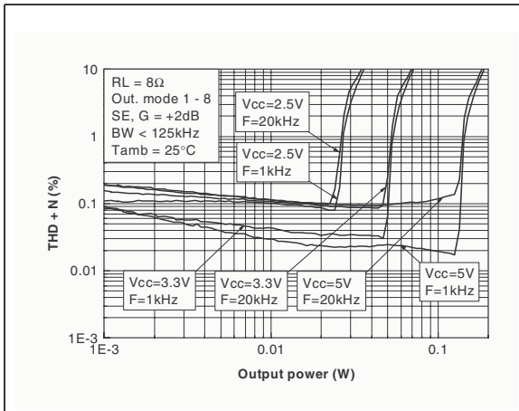
Figure 3. THD+N vs. output power
