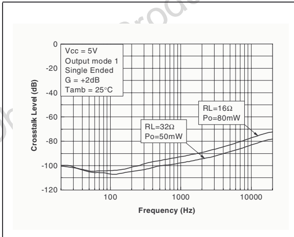
Figure 41. Crosstalk vs. frequency
