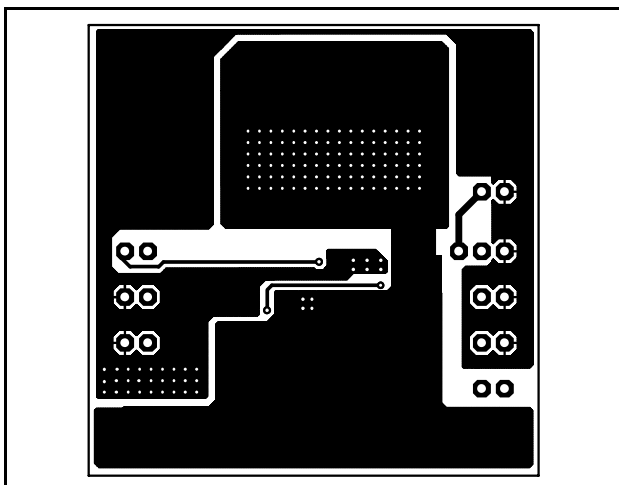
Figure 73: Bottom layer
