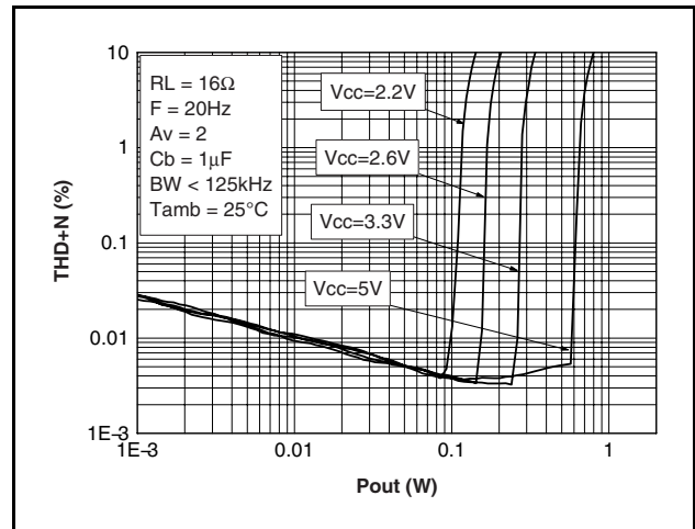
Figure 43: THD+N vs. output power
