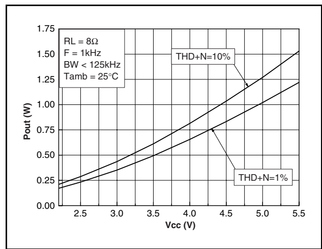
Figure 25: Output power vs. power supply voltage
