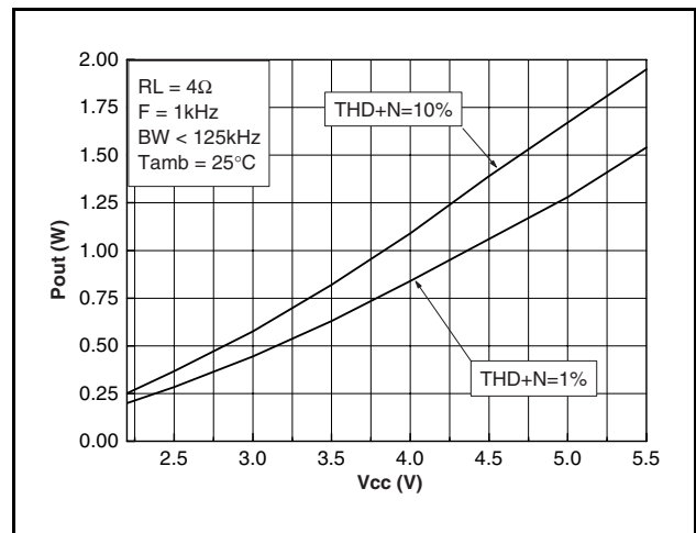
Figure 25: Output power vs. power supply voltage
