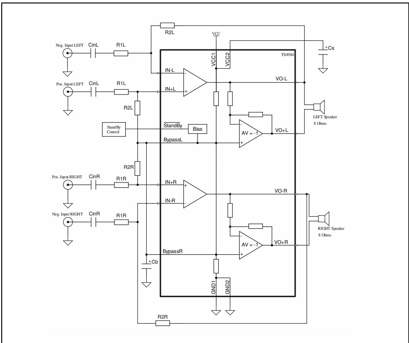
Figure 69: Differential input amplifier configuration
