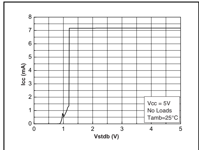
Figure 37: Current consumption vs. standby voltage at Vcc=5V
