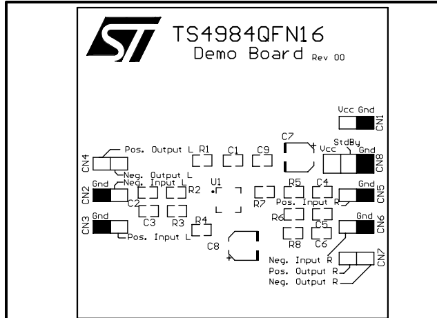
Figure 71: Components location
