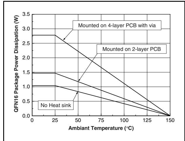
Figure 63: Power derating curves
