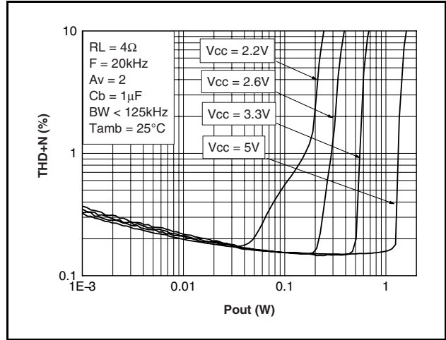
Figure 48: THD+N vs. output power
