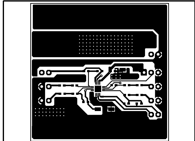
Figure 72: Top layer
