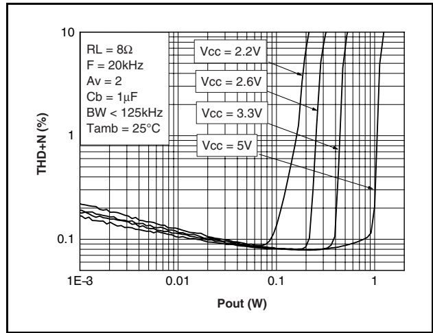
Figure 49: THD+N vs. output power
