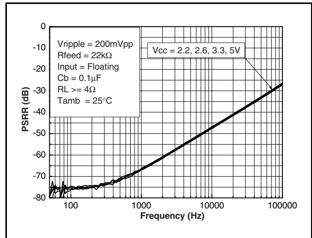
Figure 13: Power supply rejection ratio (PSRR) vs. frequency
