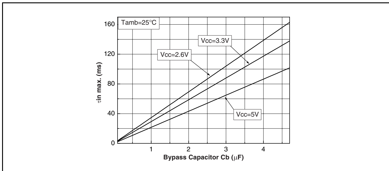
Figure 68: \tau_{in} max. versus bypass capacitor
