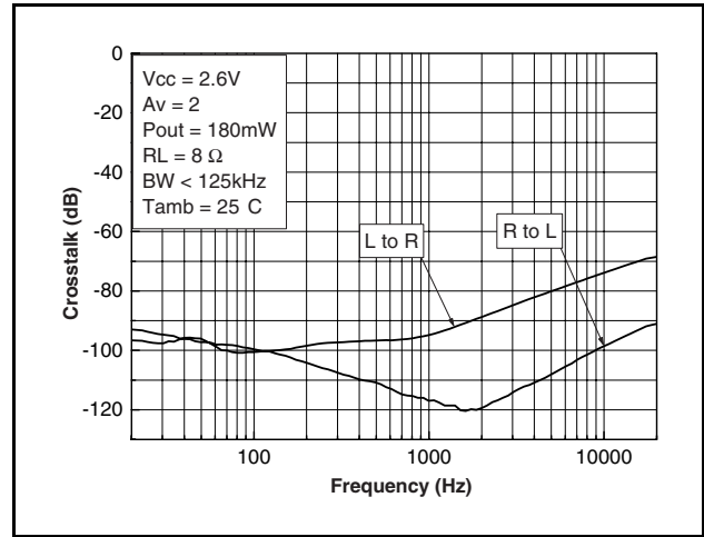
Figure 60: Crosstalk vs. frequency
