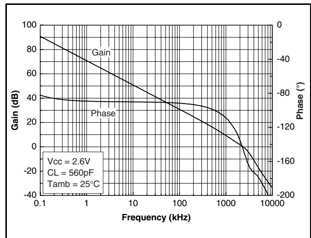
Figure 7: Open loop frequency response
