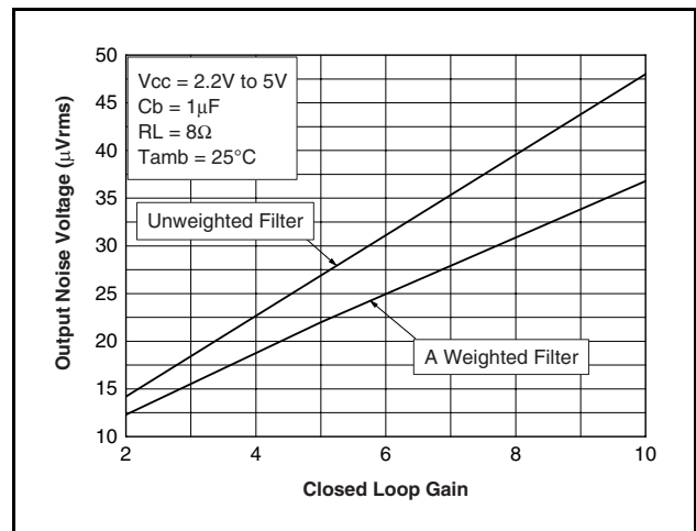
Figure 61: Output noise voltage, device ON
