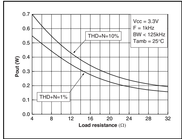
Figure 30: Output power vs. load resistor
