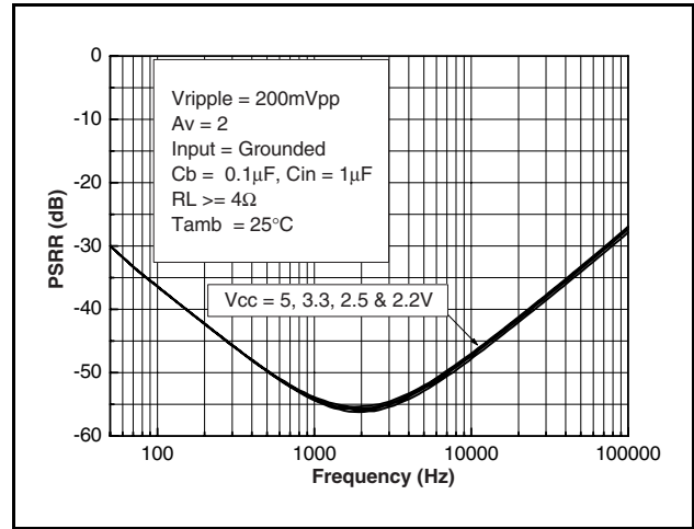
Figure 12: Power supply rejection ratio (PSRR) vs. frequency
