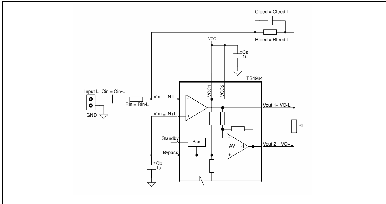
Figure 64: Typical application schematic - left channel
