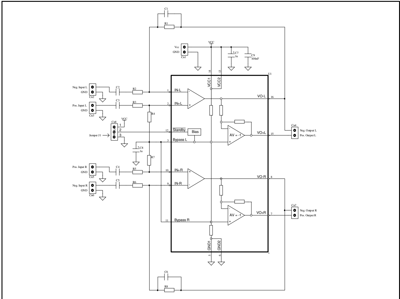
Figure 70: Demoboard schematic
