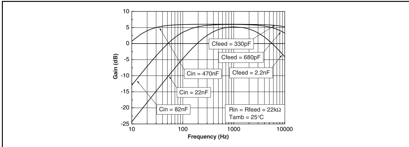
Figure 65: Frequency response gain versus C_{in} & C_{feed}
