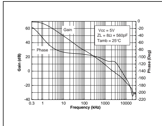
Fig. 4 : Open Loop Frequency Response
