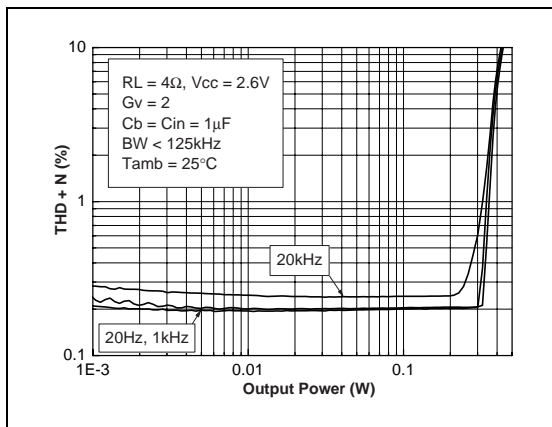
Fig. 25 : THD + N vs Output Power
