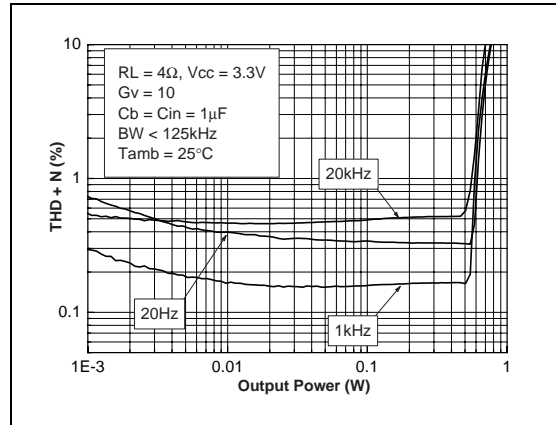
Fig. 26 : THD + N vs Output Power
