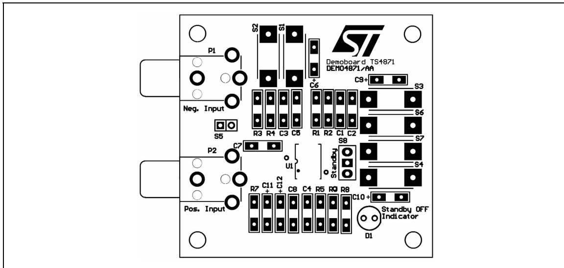
Fig. 82 : SO8 & MiniSO8 Demoboard Components Side
