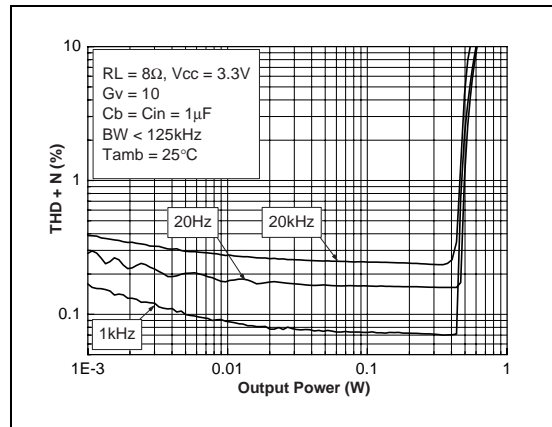
Fig. 32 : THD + N vs Output Power
