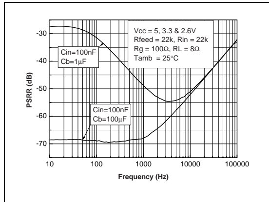
Fig. 85 : PSRR changes with Cb
