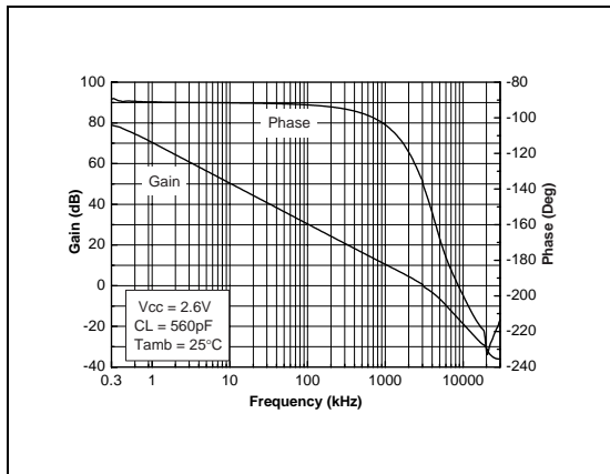
Fig. 9 : Open Loop Frequency Response
