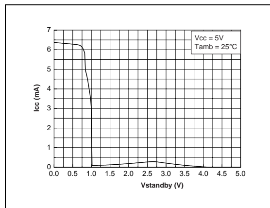
Fig. 74 : Current Consumption vs Standby Voltage @ Vcc = 5V
