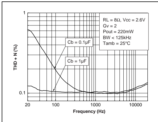
Fig. 61 : THD + N vs Frequency
