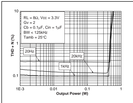
Fig. 37 : THD + N vs Output Power
