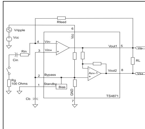
Fig. 86 : PSRR measurement schematic
