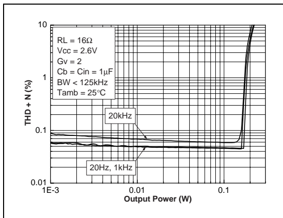
Fig. 43 : THD + N vs Output Power
