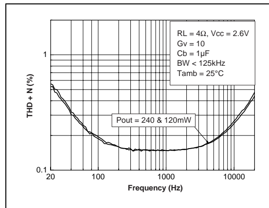
Fig. 50 : THD + N vs Frequency
