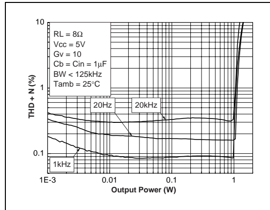
Fig. 30 : THD + N vs Output Power
