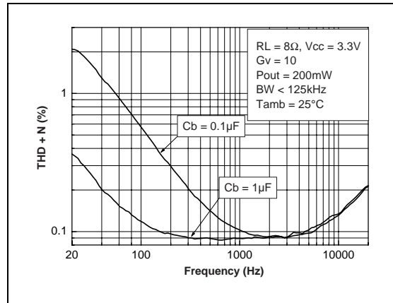
Fig. 60 : THD + N vs Frequency
