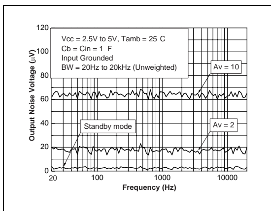
Fig. 79 : V_{out1}+V_{out2} Unweighted Noise Floor
