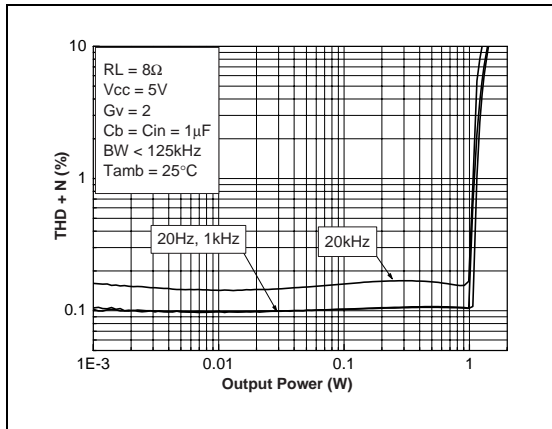
Fig. 29 : THD + N vs Output Power
