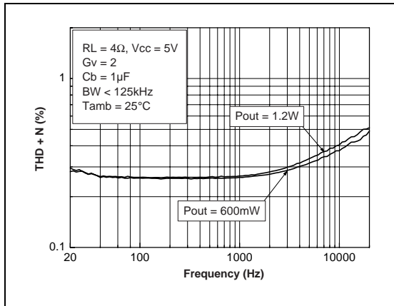
Fig. 47 : THD + N vs Frequency
