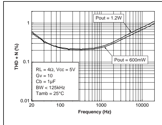
Fig. 48 : THD + N vs Frequency
