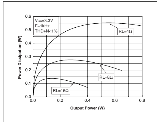
Fig. 20 : Power Derating Curves
