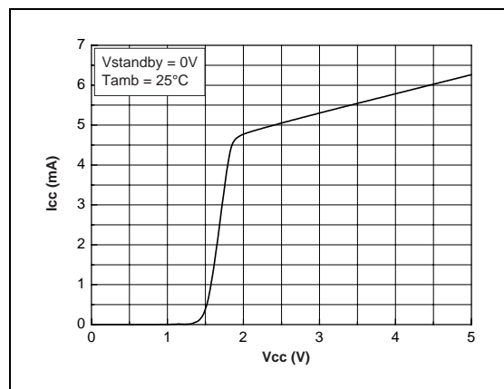
Fig. 72 : Current Consumption vs Power Supply Voltage
