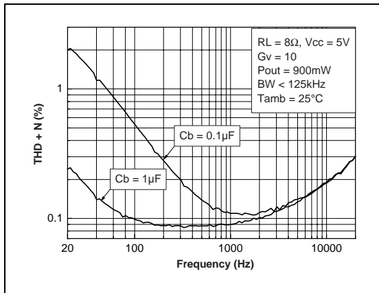
Fig. 55 : THD + N vs Frequency
