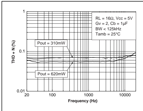
Fig. 65 : THD + N vs Frequency
