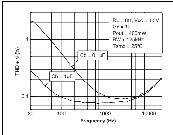
Fig. 59 : THD + N vs Frequency
