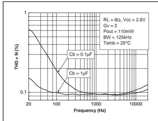
Fig. 62 : THD + N vs Frequency
