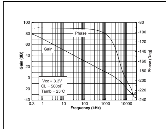
Fig. 8 : Open Loop Frequency Response
