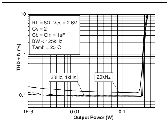
Fig. 31 : THD + N vs Output Power
