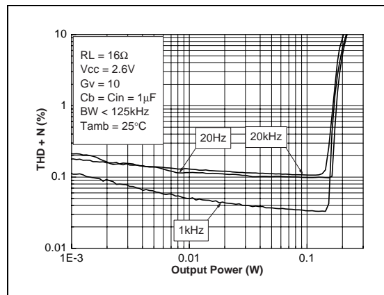
Fig. 44 : THD + N vs Output Power
