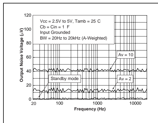
Fig. 80 : V_{out1}+V_{out2} A-weighted Noise Floor
