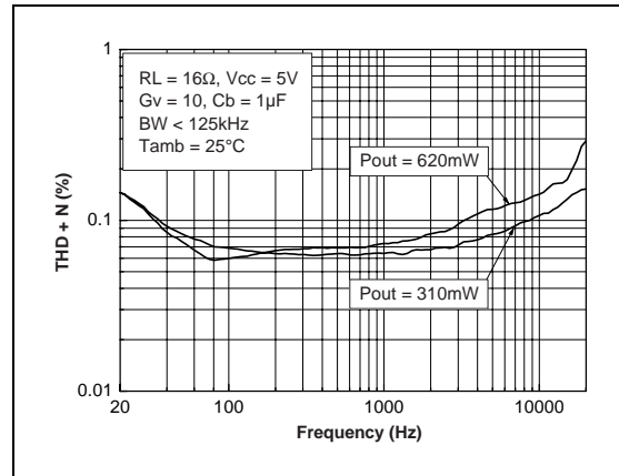
Fig. 66 : THD + N vs Frequency
