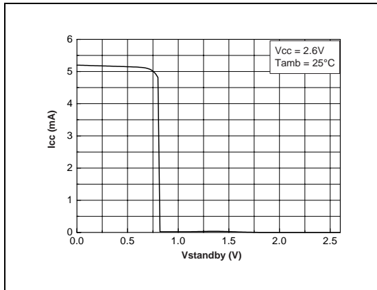
Fig. 75 : Current Consumption vs Standby Voltage @ V_{CC} = 2.6V
