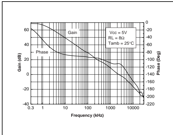
Fig. 3 : Open Loop Frequency Response
