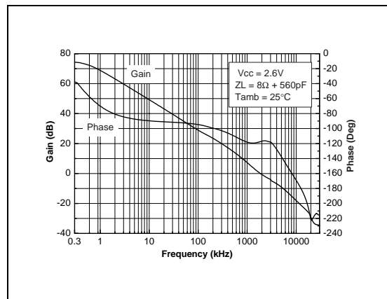
Fig. 6 : Open Loop Frequency Response
