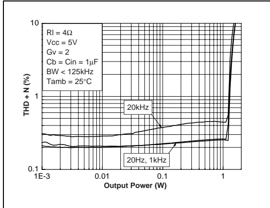
Fig. 23 : THD + N vs Output Power
