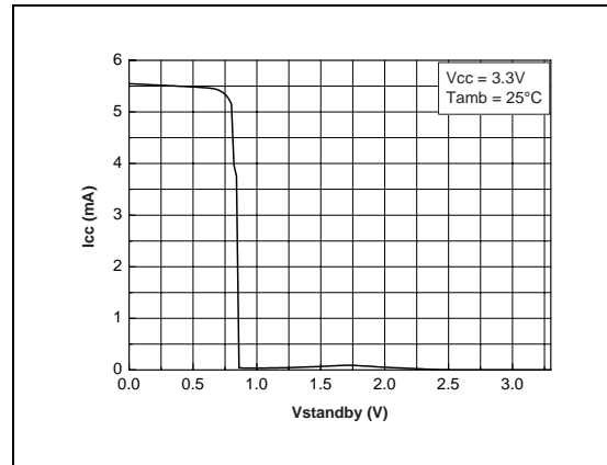
Fig. 76 : Current Consumption vs Standby Voltage @ V_{CC} = 3.3V
