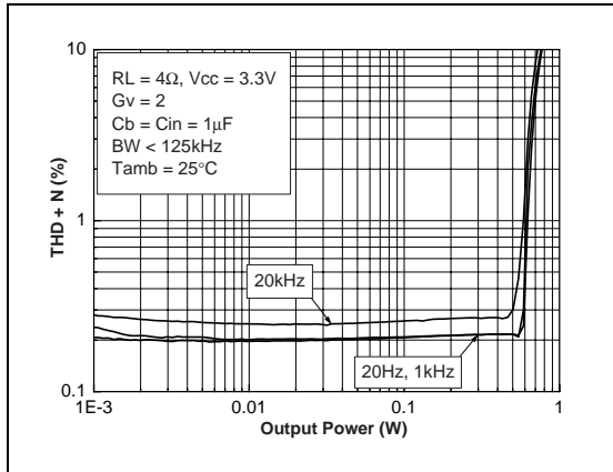
Fig. 25 : THD + N vs Output Power
