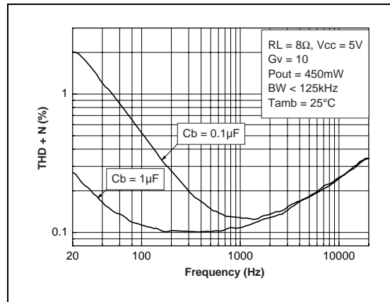
Fig. 56 : THD + N vs Frequency
