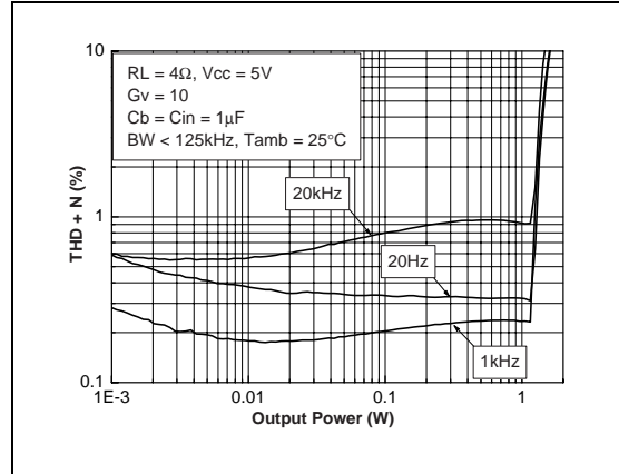
Fig. 24 : THD + N vs Output Power
