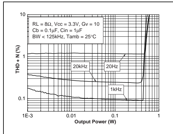
Fig. 38 : THD + N vs Output Power
