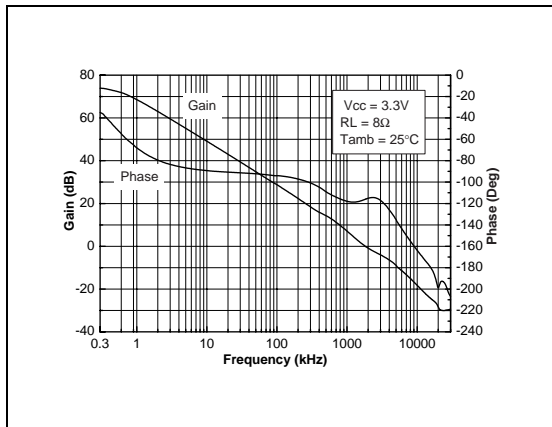
Fig. 5 : Open Loop Frequency Response
