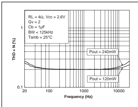
Fig. 49 : THD + N vs Frequency
