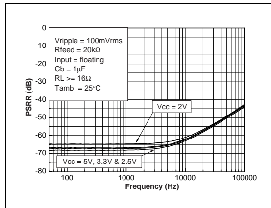
Fig. 52: PSRR vs Power Supply Voltage
