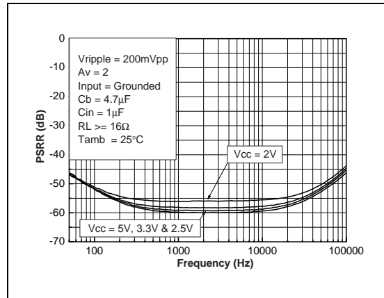
Fig. 54: PSRR vs Bypass Capacitor
