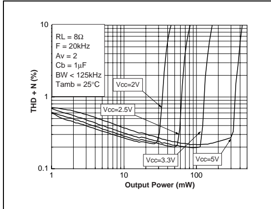
Fig. 43: THD + N vs Output Power
