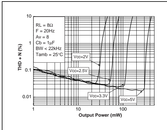
Fig. 79: THD + N vs Output Power
