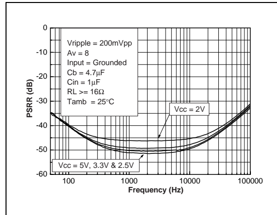
Fig. 96: PSRR vs Bypass Capacitor
