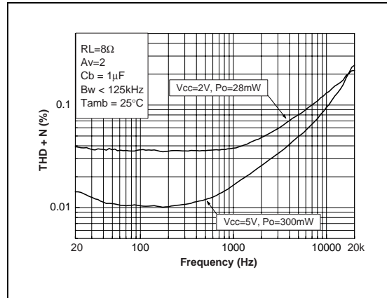
Fig. 46: THD + N vs Frequency
