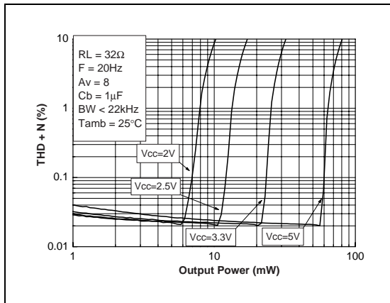
Fig. 81: THD + N vs Output Power
