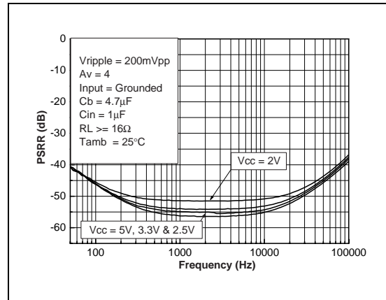
Fig. 75: PSRR vs Bypass Capacitor
