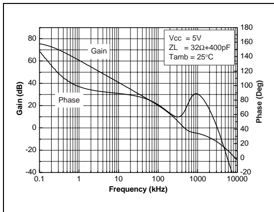
Fig. 11: Open Loop Gain and Phase vs Frequency
