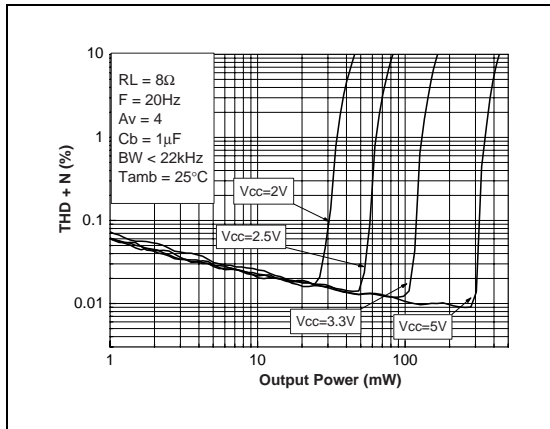
Fig. 58: THD + N vs Output Power
