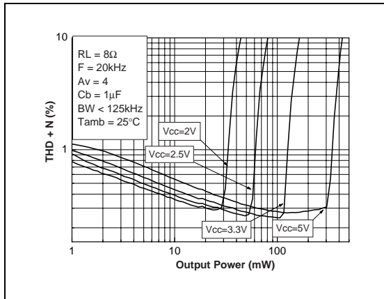
Fig. 64: THD + N vs Output Power
