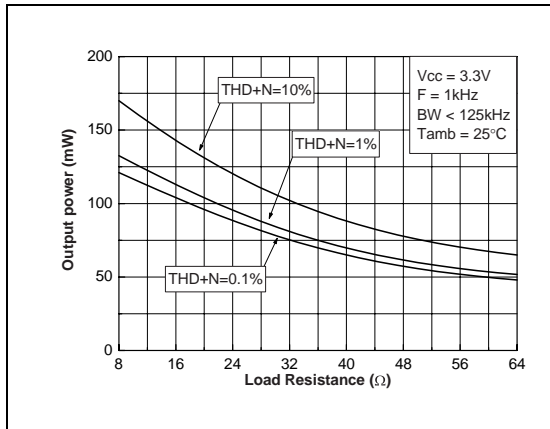
Fig. 27: Output Power vs Load Resistor
