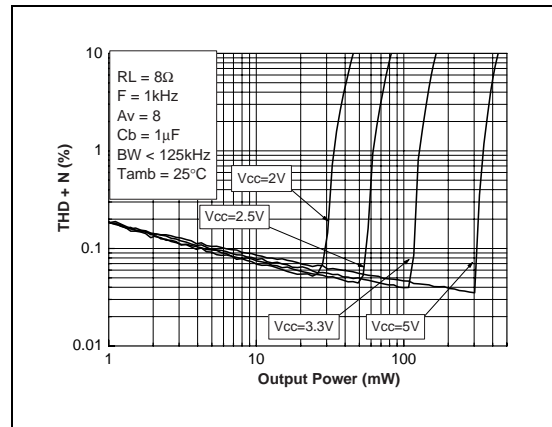
Fig. 82: THD + N vs Output Power
