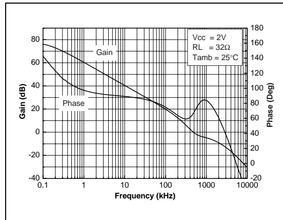
Fig. 12: Open Loop Gain and Phase vs Frequency
