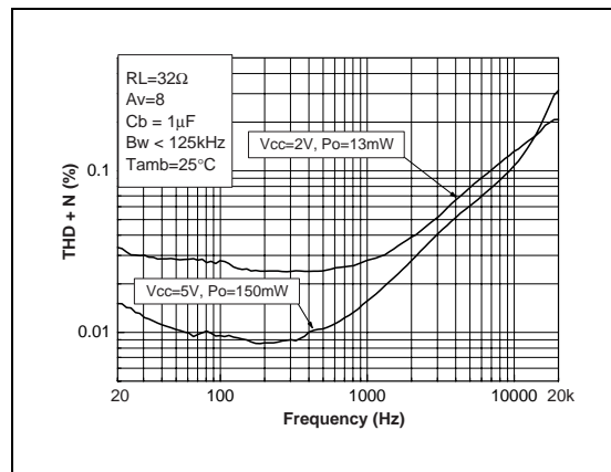
Fig. 88: THD + N vs Frequency
