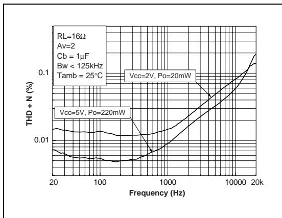
Fig. 45: THD + N vs Frequency
