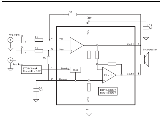
Fig. 98 : Differential Input Amplifier Configuration
