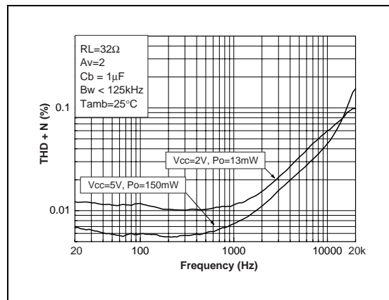
Fig. 46: THD + N vs Frequency
