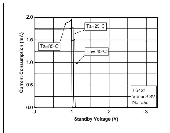
Fig. 18: Current Consumption vs Standby Voltage
