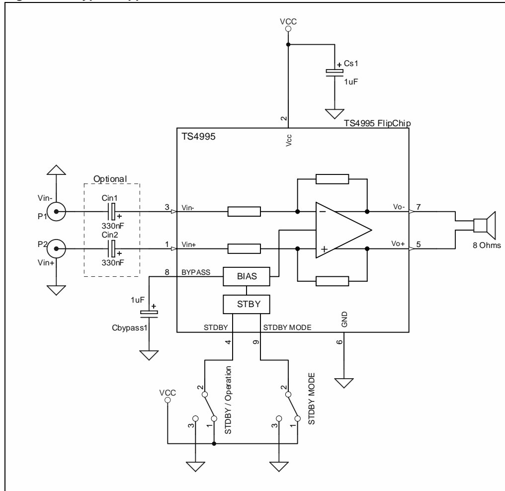
Figure 1. Typical application
