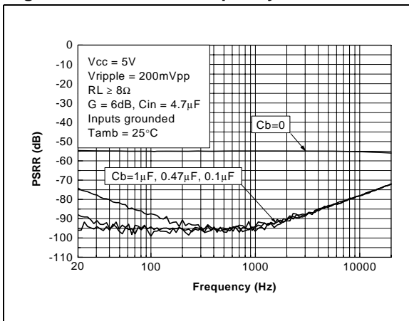
Figure 36. PSSR vs. frequency
