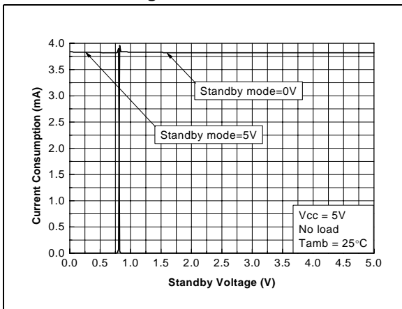
Figure 48. Current consumption vs. standby voltage
