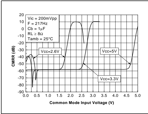
Figure 44. CMRR vs. common mode input voltage
