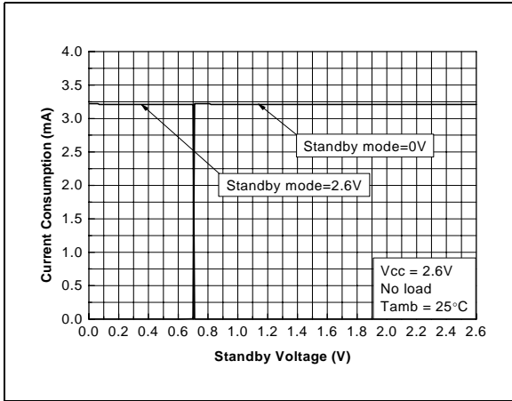
Figure 50. Current consumption vs. standby voltage
