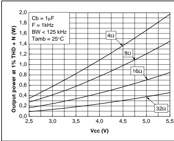
Figure 26. Output power vs. power supply voltage
