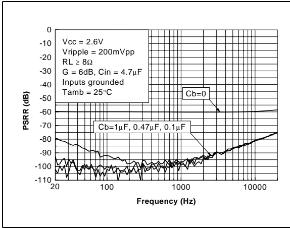
Figure 32. PSSR vs. frequency
