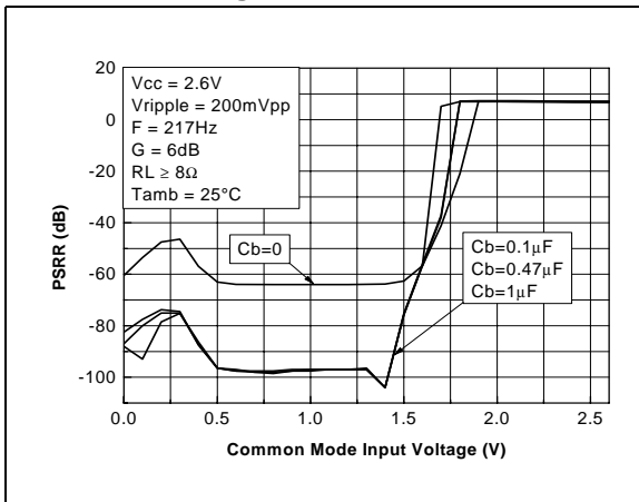
Figure 40. PSSR vs. common mode input voltage
