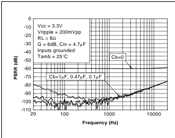
Figure 34. PSSR vs. frequency
