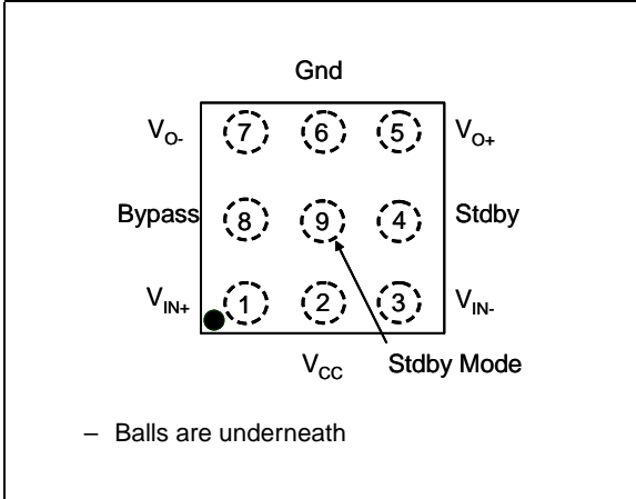
Figure 61. Pin out (top view)
