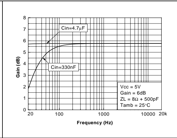
Figure 53. Frequency response
