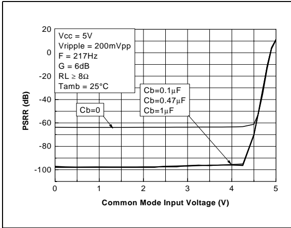
Figure 38. PSSR vs. common mode input voltage
