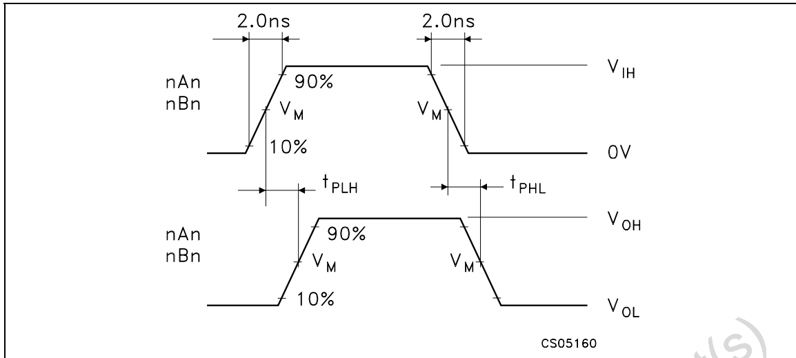
WAVEFORM 1: PROPAGATION DELAYS (f=1MHz; 50% duty cycle)
