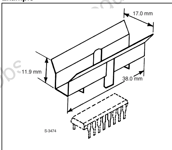
Figure 12. External Heatsink Mounting Example
