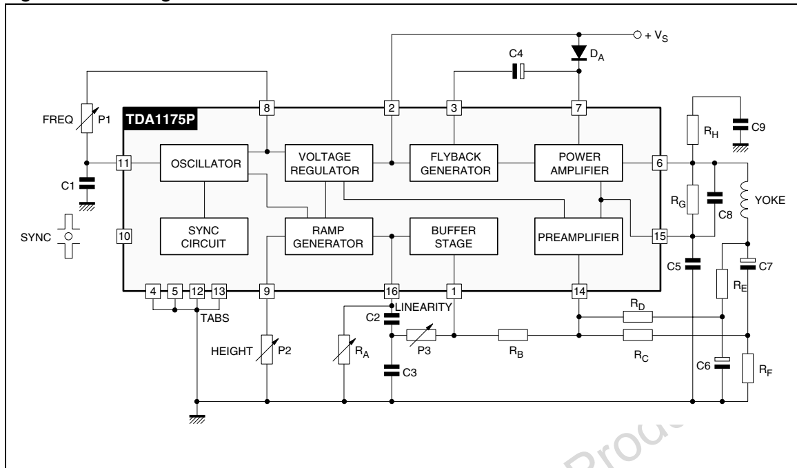
Figure 3. Block Diagram
