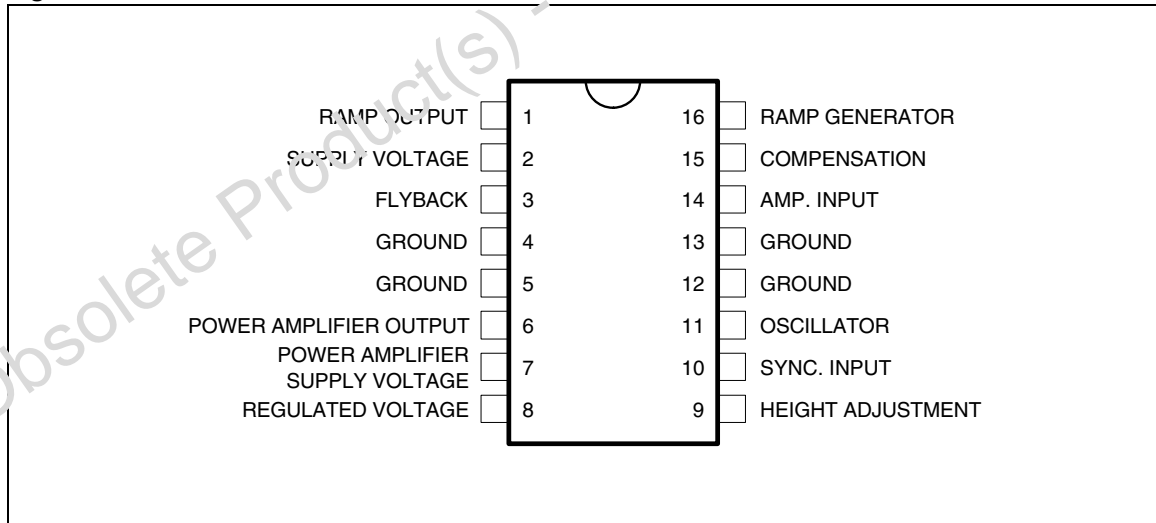
Figure 2. Pin Connections
