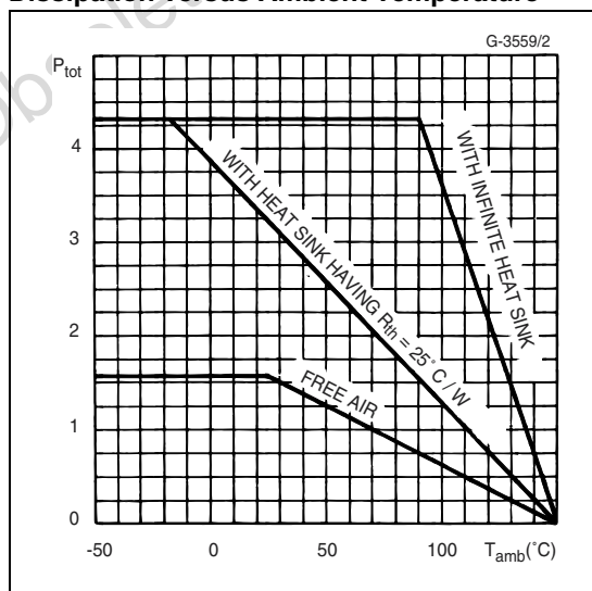
Figure 14. Maximum Allowable Power Dissipation versus Ambient Temperature
