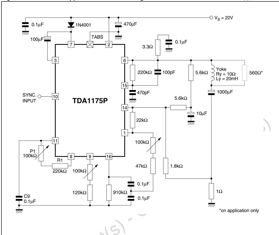
Figure 8. AC Test and Application Circuit for Large Screen B/W TV Set 10Ω/20mH/1A pp
