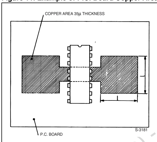
Figure 11. Example of P.C. Board Copper Area
