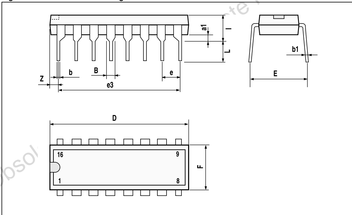
Figure 15. POWERDIP16 - Package Dimensions
