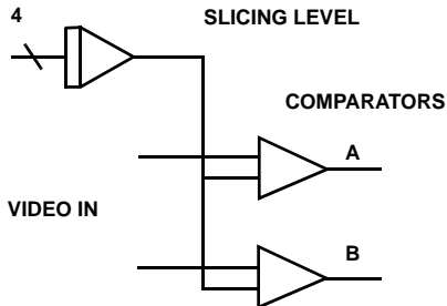
FIGURE 15. DELAY DETECTOR
