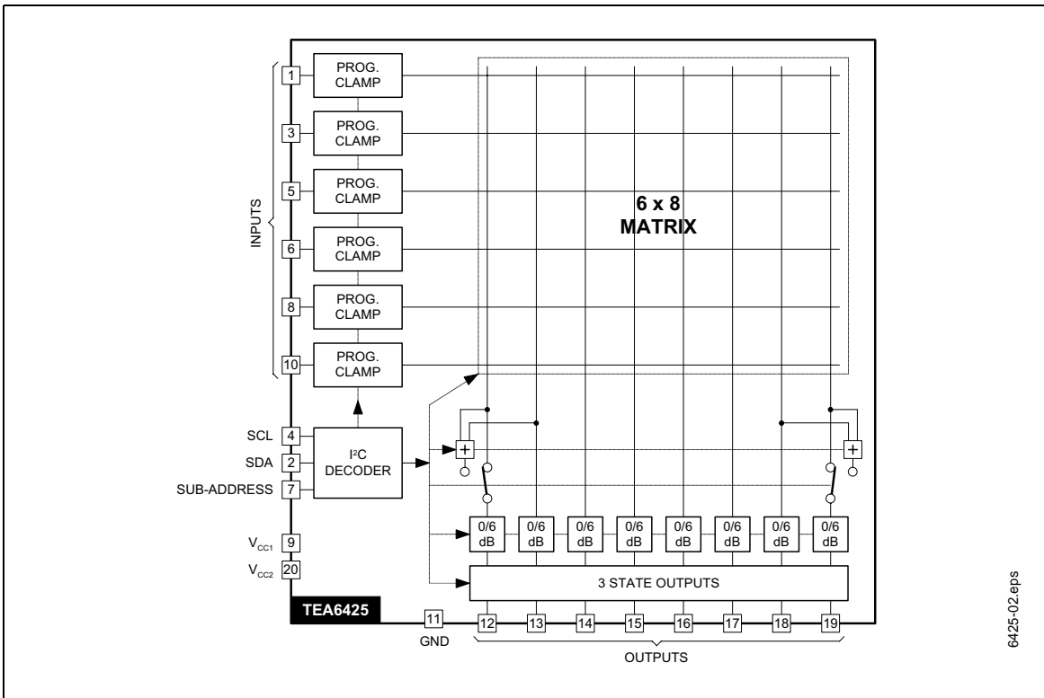
Figure 2. Block Diagram
