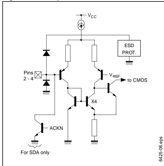
Figure 8. Bus Inputs
