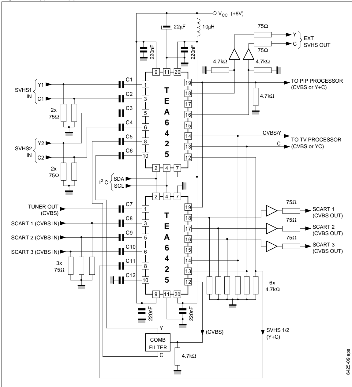
Figure 9. Typical Application
