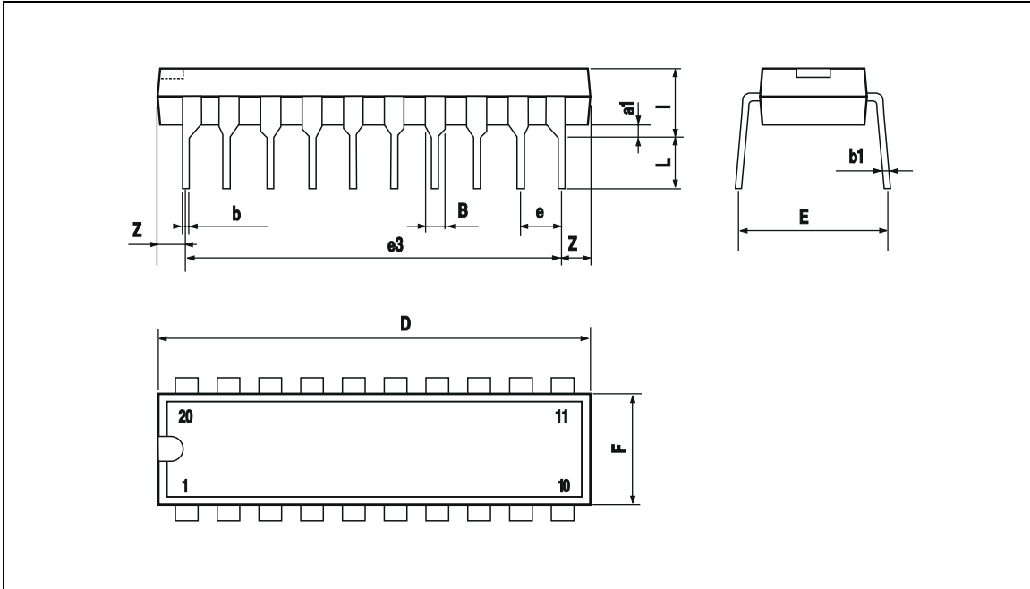
Figure 10. 20-Pin Package
