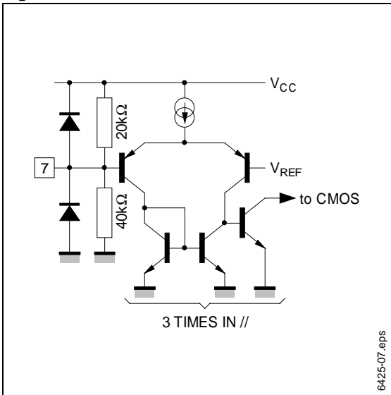
Figure 7. PROG Pin
