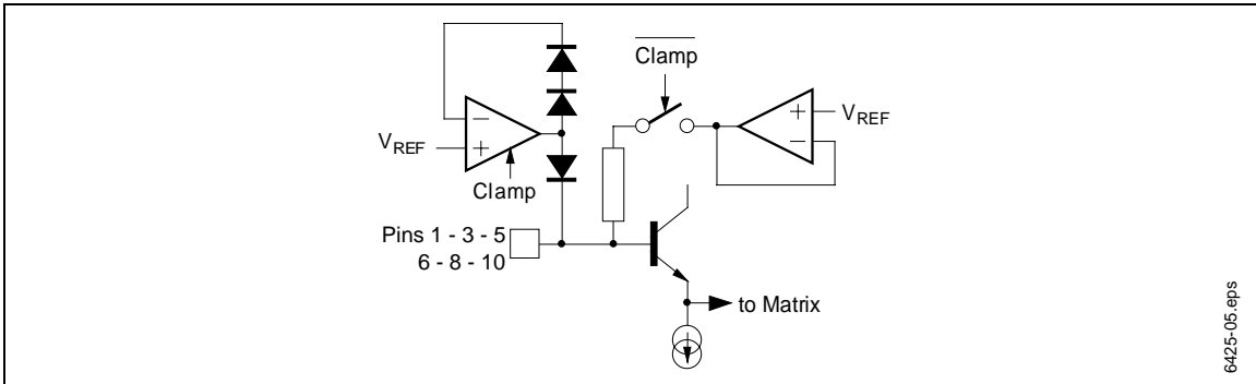
Figure 6. Video OUT
