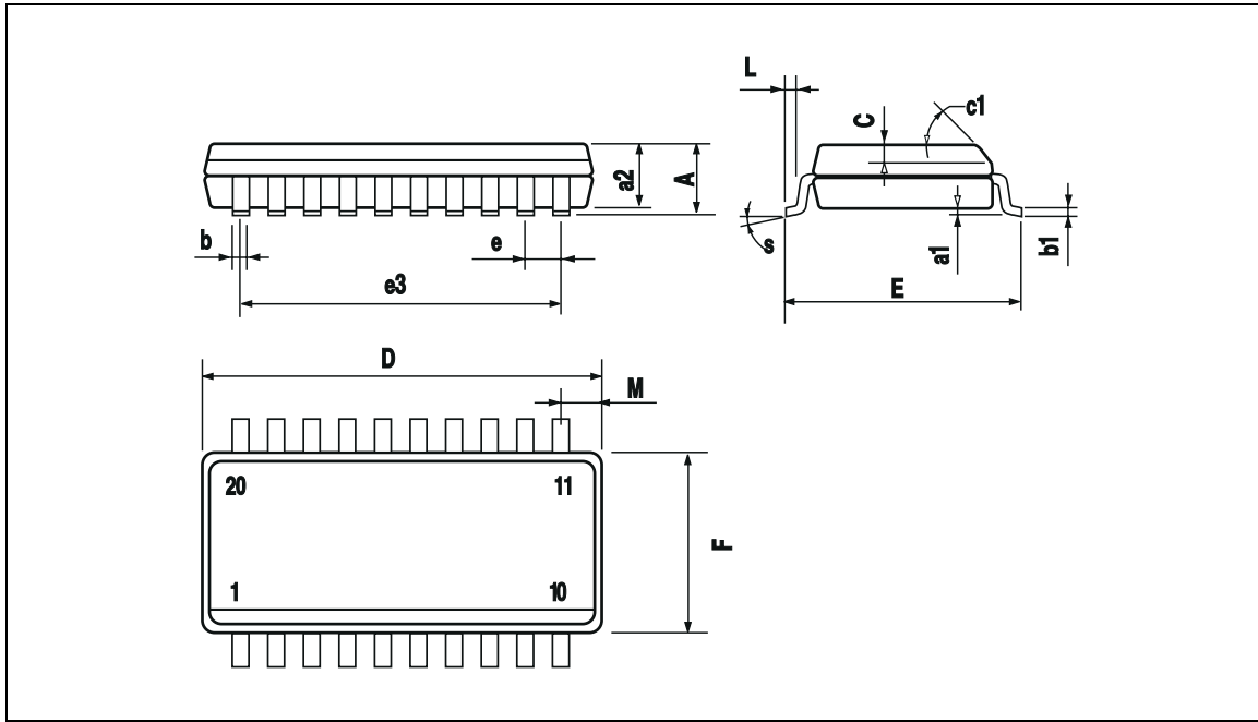
Figure 11. 20-Pin Package
