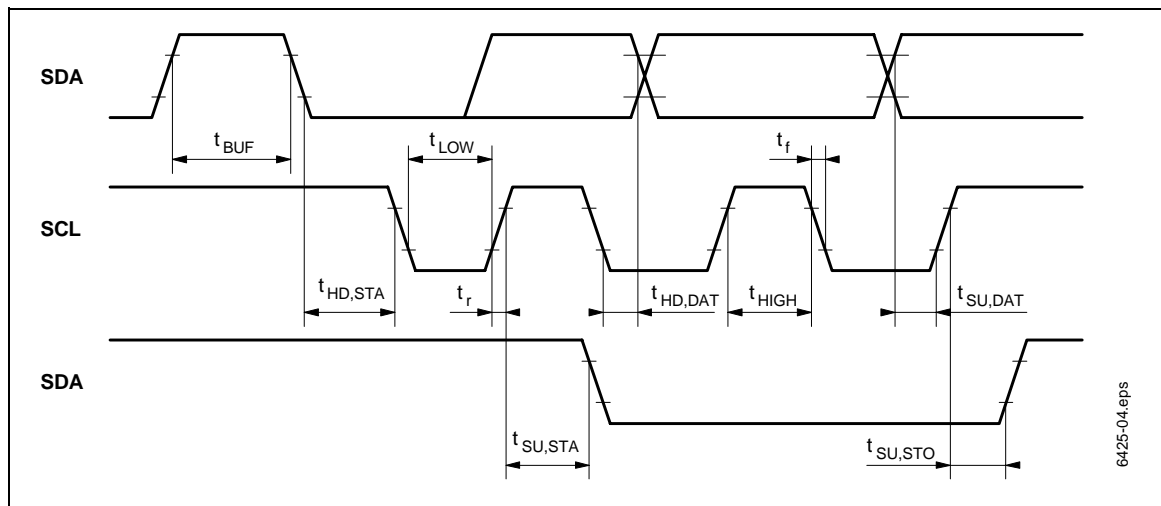
Figure 4. I 2 C Bus Timing
