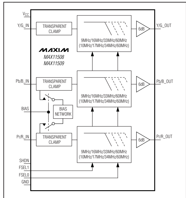
Figure 1. Block Diagram
