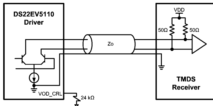
FIGURE 9. DC Coupled Application
