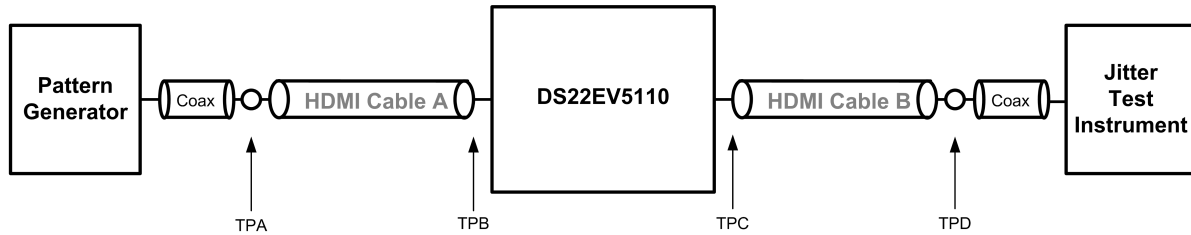
FIGURE 13. Simplified Test Setup as a Single Repeater
