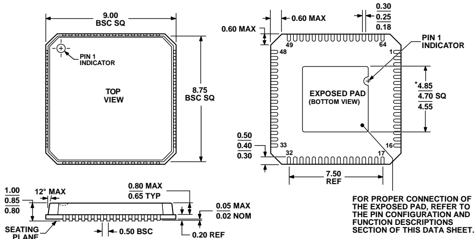
*COMPLIANT TO JEDEC STANDARDS MO-220-VMM4-4 EXCEPT FOR EXPOSED PAD DIMENSION Figure 6. 64-Lead Lead Frame Chip Scale Package [LFCSP_VQ] 9 mm x 9 mm Body, Very Thin Quad (CP-64-1) Dimensions shown in millimeters
