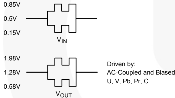
Figure 12. Typical Voltage Levels
