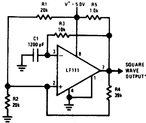
100 kHz Free Running Multivibrator
