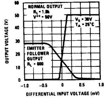
Transfer Function
