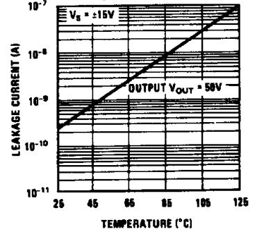
Leakage Currents
