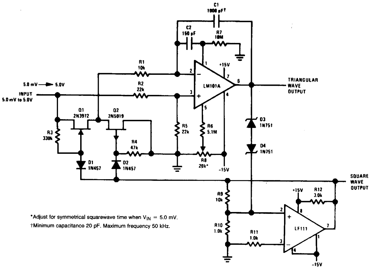
10 Hz to 10 kHz Voltage Controlled Oscillator
