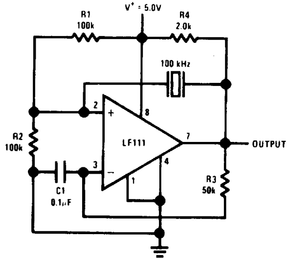
Crystal Oscillator
