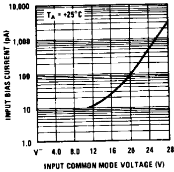
Input Bias Current vs Common Mode
