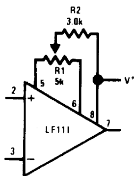
Offset Balancing
