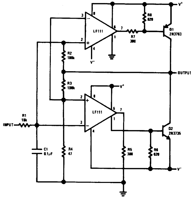
Switching Power Amplifier
