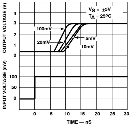
Figure 3. Response Time for Various Input Overdrives
