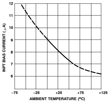
Figure 9. Input Bias Current vs. Ambient Temperature
