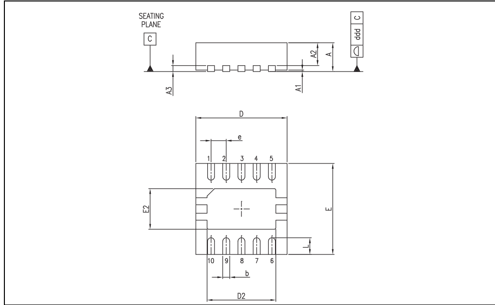
Figure 72. DFN8 3x3x0.90mm package mechanical drawing (pitch 0.5mm)
