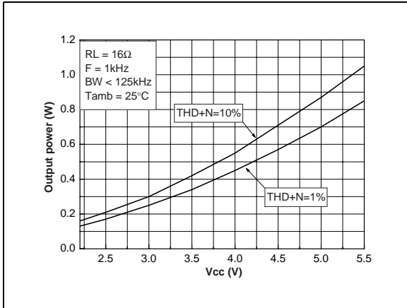
Figure 26. Output power vs. power supply voltage
