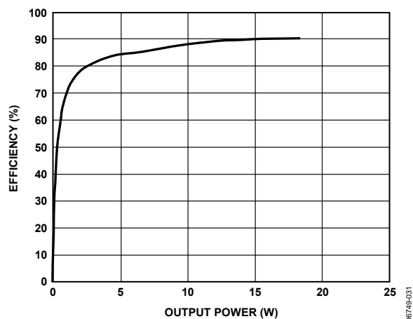
Figure 31. Efficiency vs. Output Power, 15 V, 8 Ω
