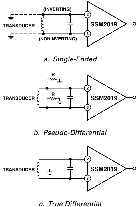
Figure 3. Three Ways of Interfacing Transducers for High Noise Immunity
