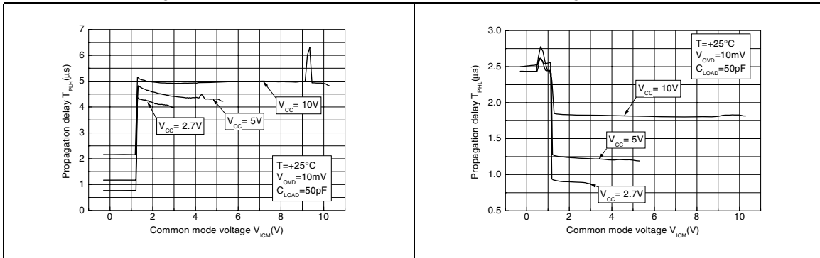
Figure 17. Propagation delay T_{PLH} versus V_{ICM} with V_{OVD} = 10mV Figure 18. Propagation delay T_{PHL} versus V_{ICM} with V_{OVD} = 10mV
