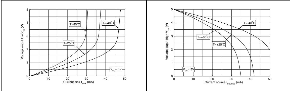
Figure 13. V_{OL} versus I_{SINK} and temperature at V_{CC} = 5V Figure 14. V_{OH} versus I_{SOURCE} and temperature at V_{CC} = 5V
