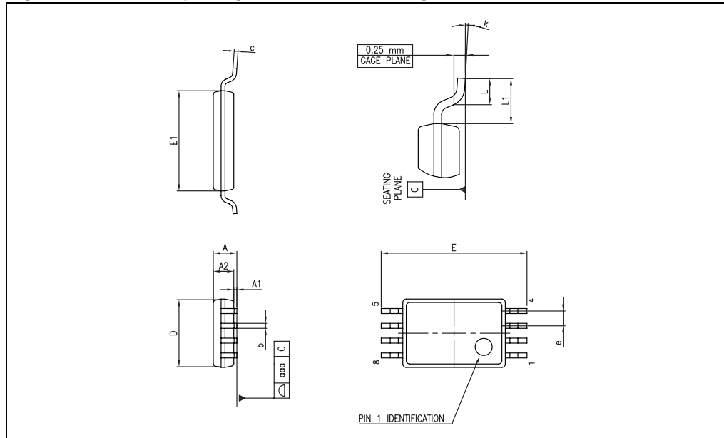
Figure 25. TSSOP8 package mechanical drawing
