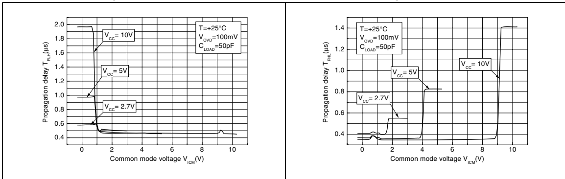
Figure 15. Propagation delay T_{PLH} versus V_{ICM} with V_{OVD} = 100mV Figure 16. Propagation delay T_{PHL} versus V_{ICM} with V_{OVD} = 100mV
