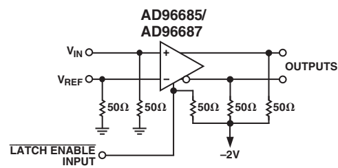
Figure 2. High Speed Sampling Circuit
