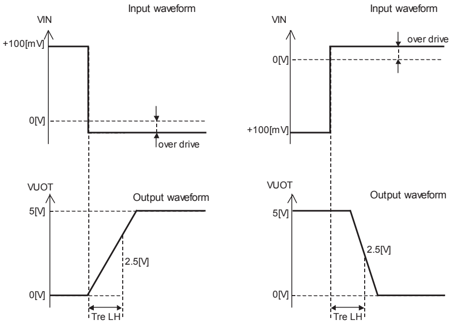
Fig.4 Response Time
