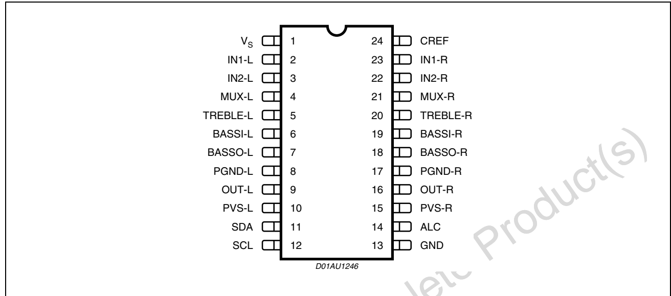
Figure 3. PIN CONNECTIONS (Top view)
