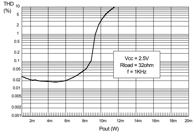
Figure 7. THD+Noise vs Amplitude @ V_{CC} 2.5V, R_{load} 32 \Omega
