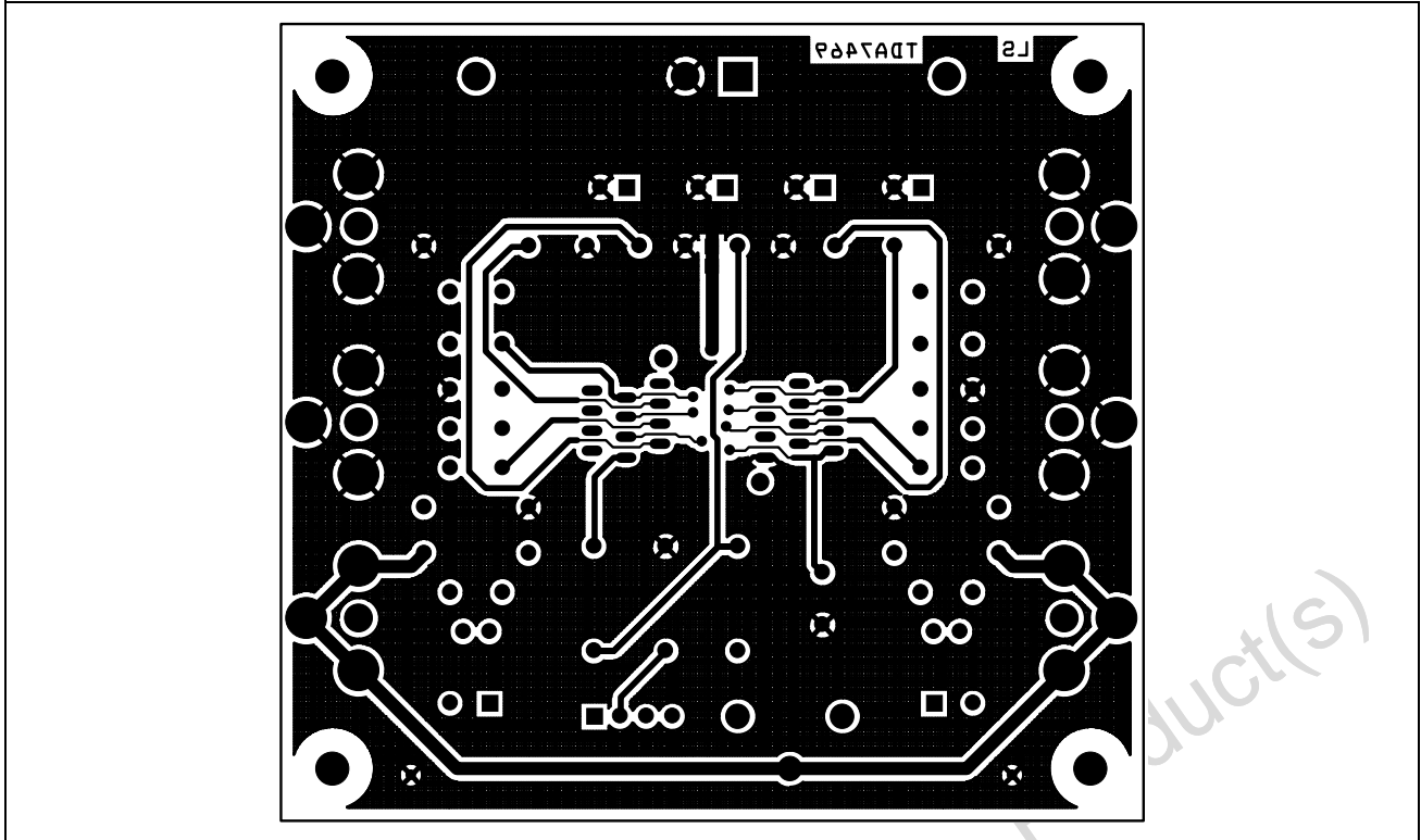
Figure 11. TDA7469 P. C. Board (Backside view)
