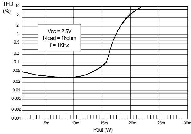
Figure 5. THD+Noise vs Amplitude @ V_{CC} 2.5V, R_{load} 16 \Omega
