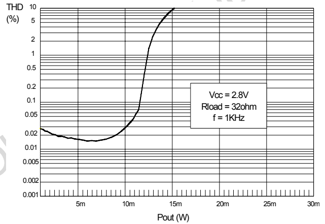
Figure 8. THD+Noise vs Amplitude @ V_{CC} 2.8V, R_{load} 32 \Omega
