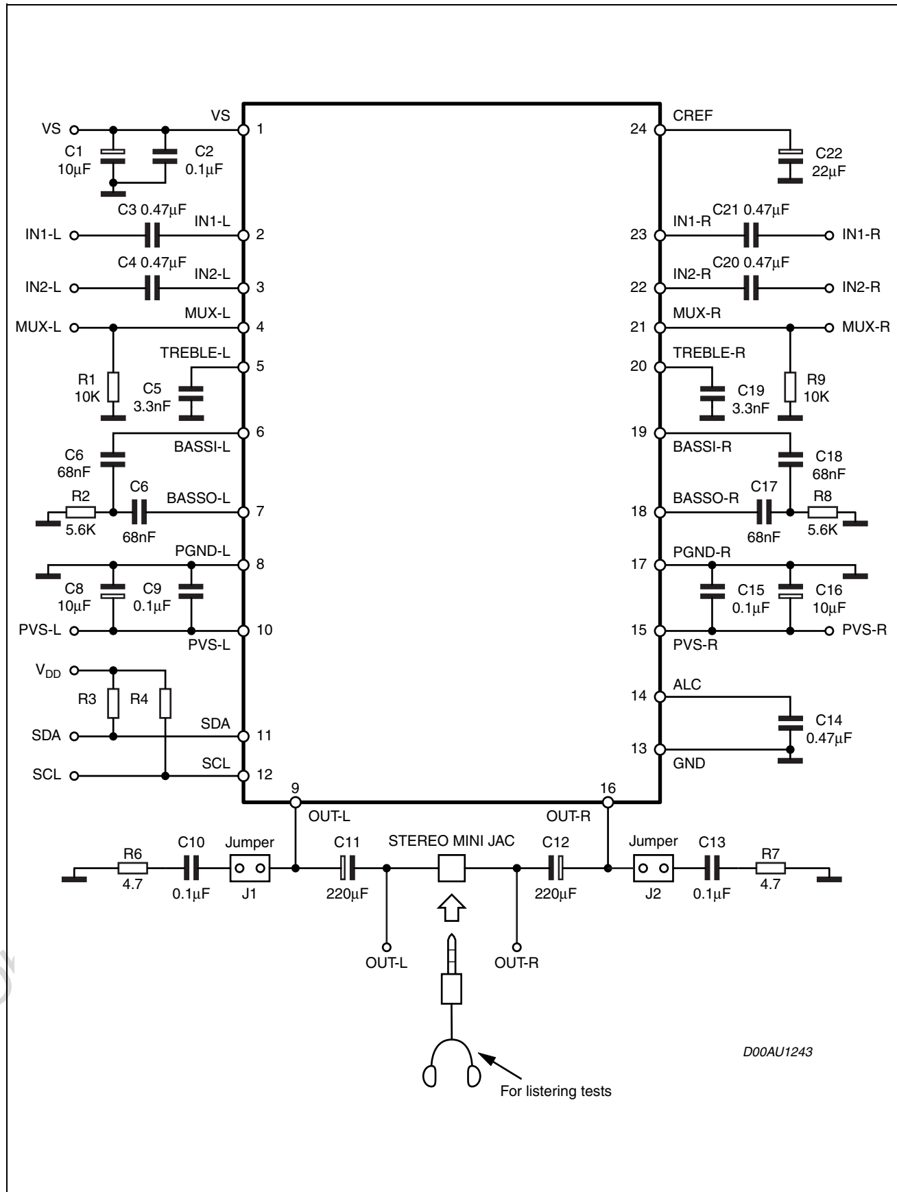
Figure 4. Typical Application Circuit (SSO24)
