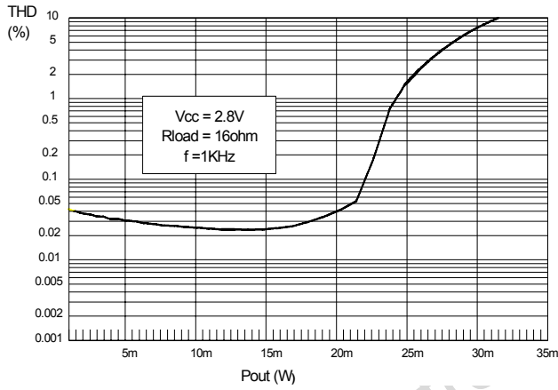
Figure 6. THD+Noise vs Amplitude @ V_{CC} 2.8V, R_{load} 16 \Omega
