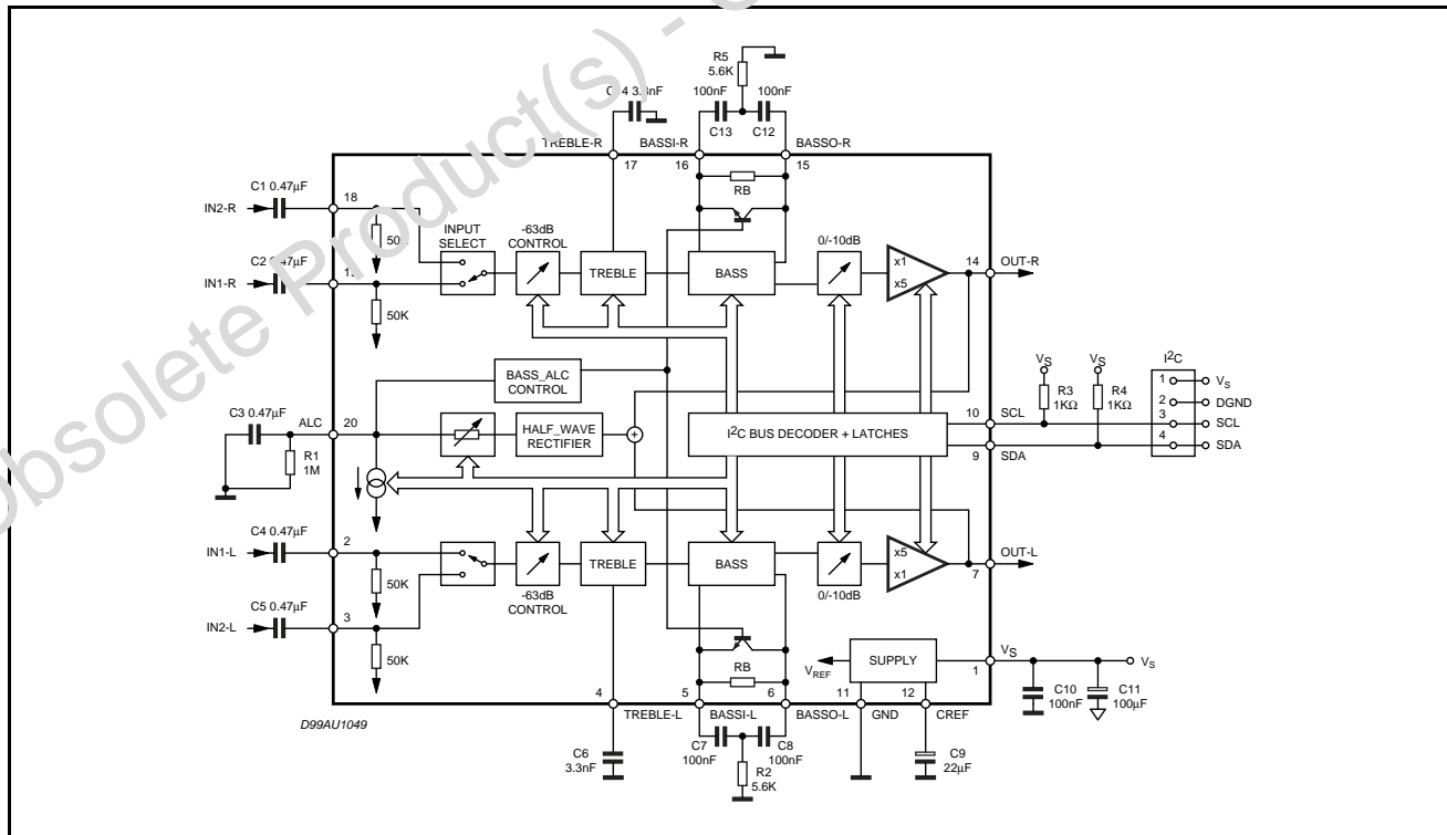
Figure 2. Application & Test Circuit
