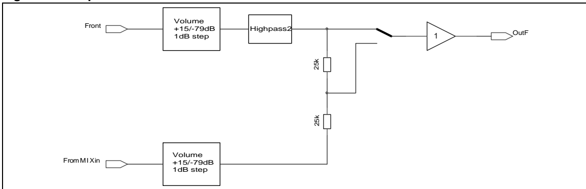
Figure 16. Output Selector
