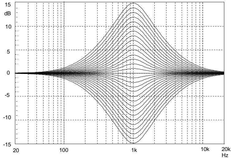
Figure 7. Equalizer filter control @ f_{Center} = 1kHz , Q = 1.0
