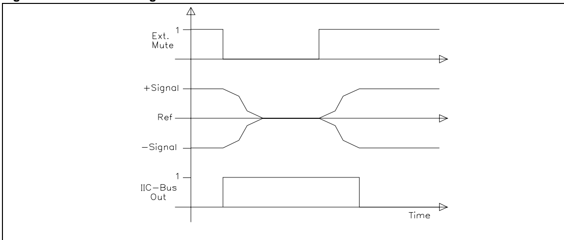
Figure 5. Soft Mute-Timing
