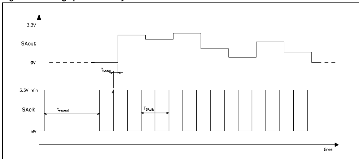
Figure 14. Timing spectrum analyzer
