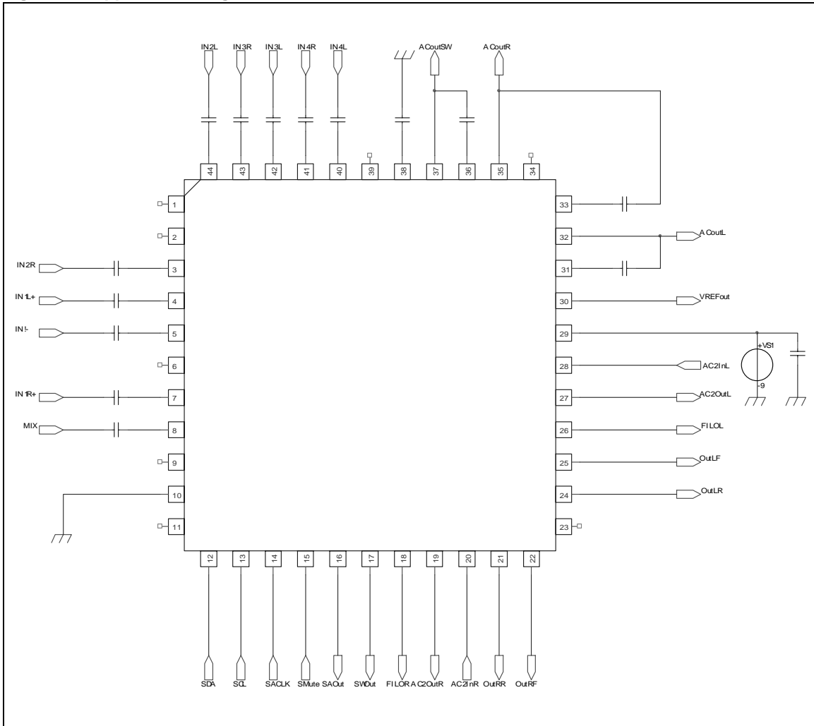
Figure 17. Application Diagram
