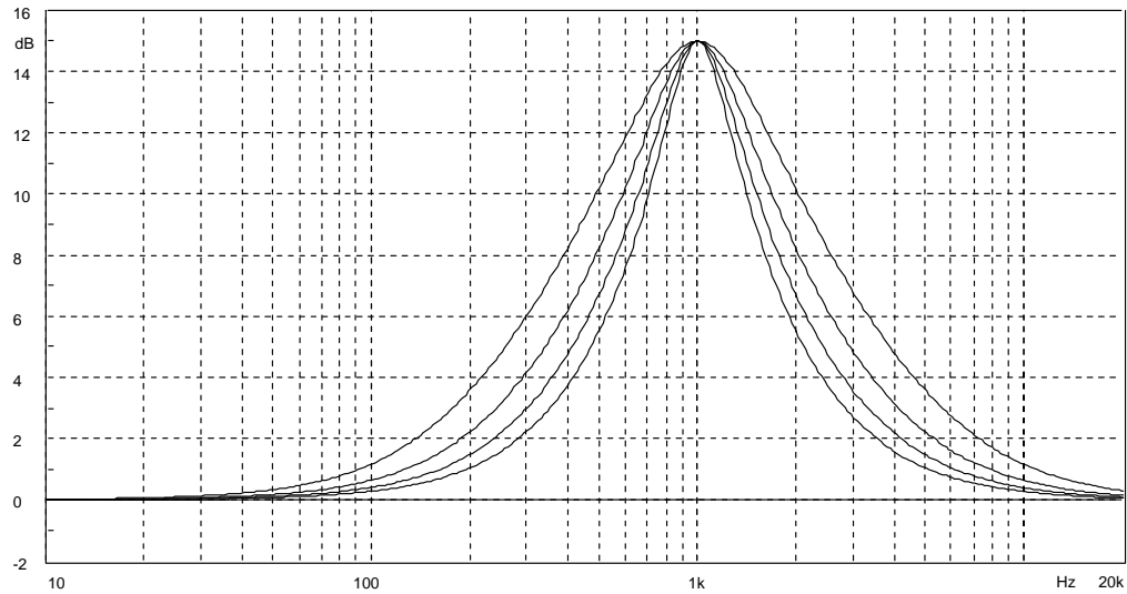
Figure 9. Quality factors @ boost = 15dB, f_{\text{Center}} = 1\text{kHz}
