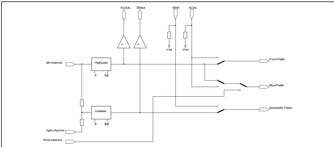
Figure 15. AC/DC-coupling
