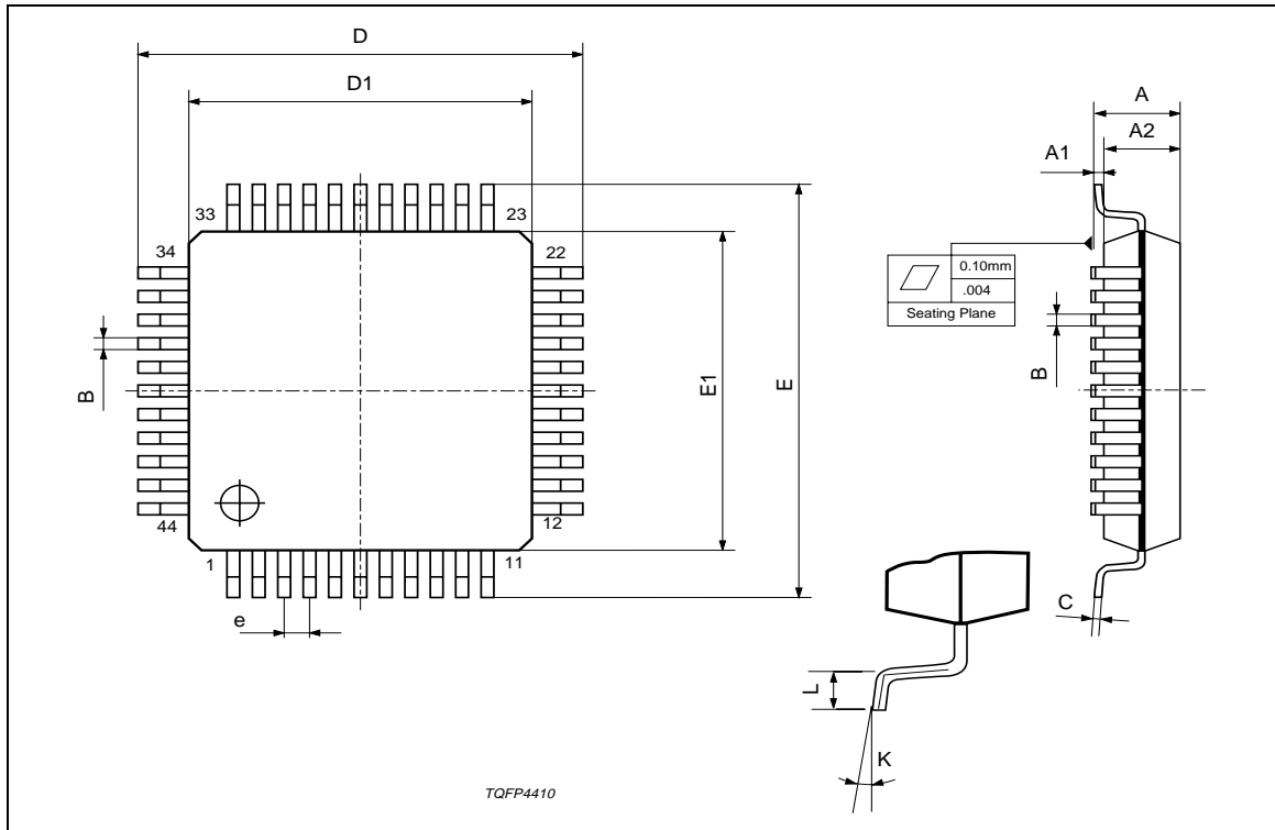
TQFP44 (10 x 10)
