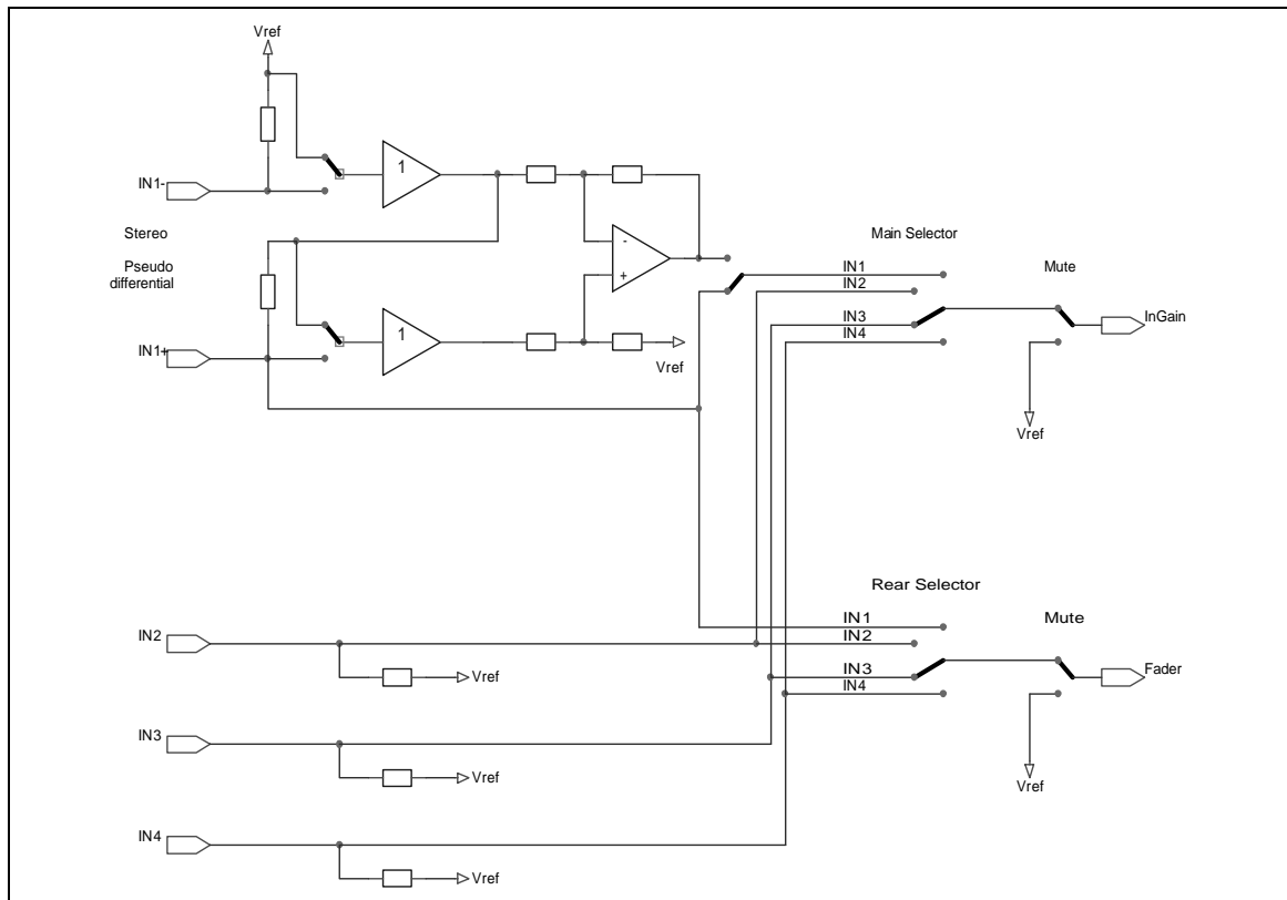
Figure 1. Input-stages
