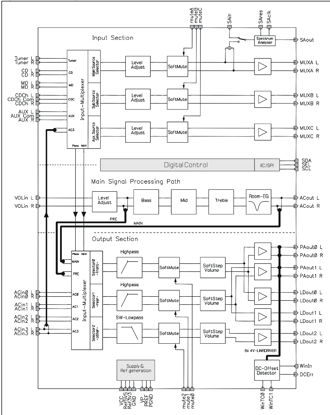
Figure 1. Block diagram
