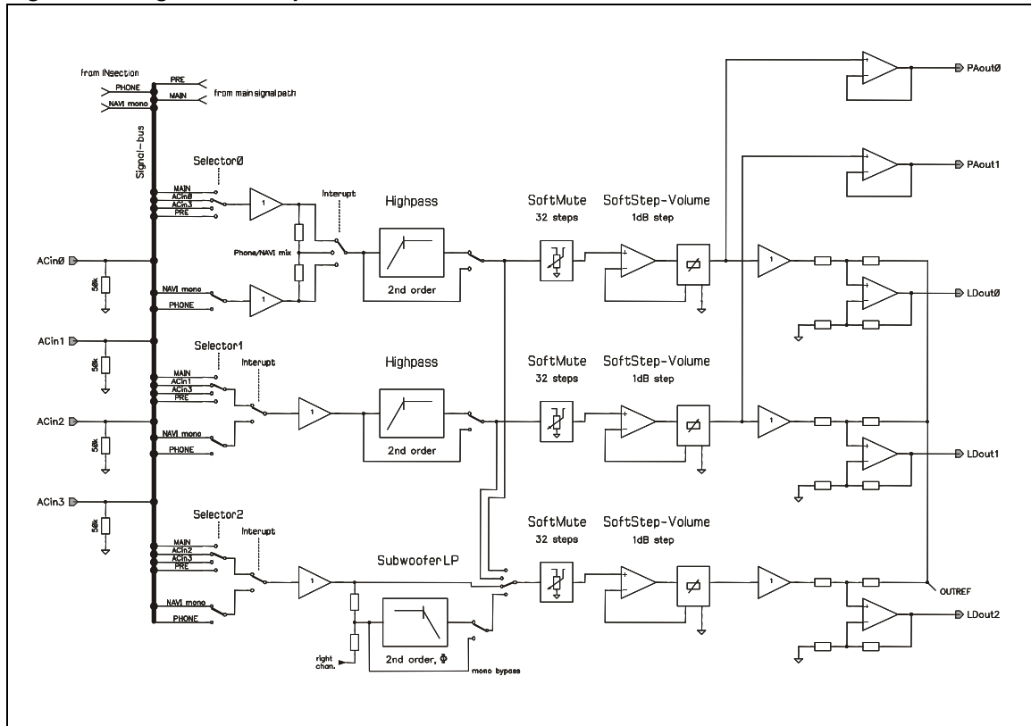
Figure 16. Signal flow output section
