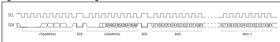
Figure 26. I 2 C bus interface diagram
