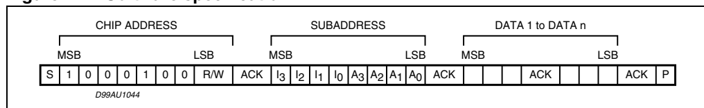
Figure 17. Software specification
