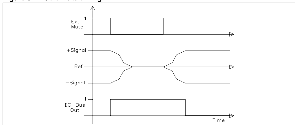
Figure 8. Soft-mute timing
