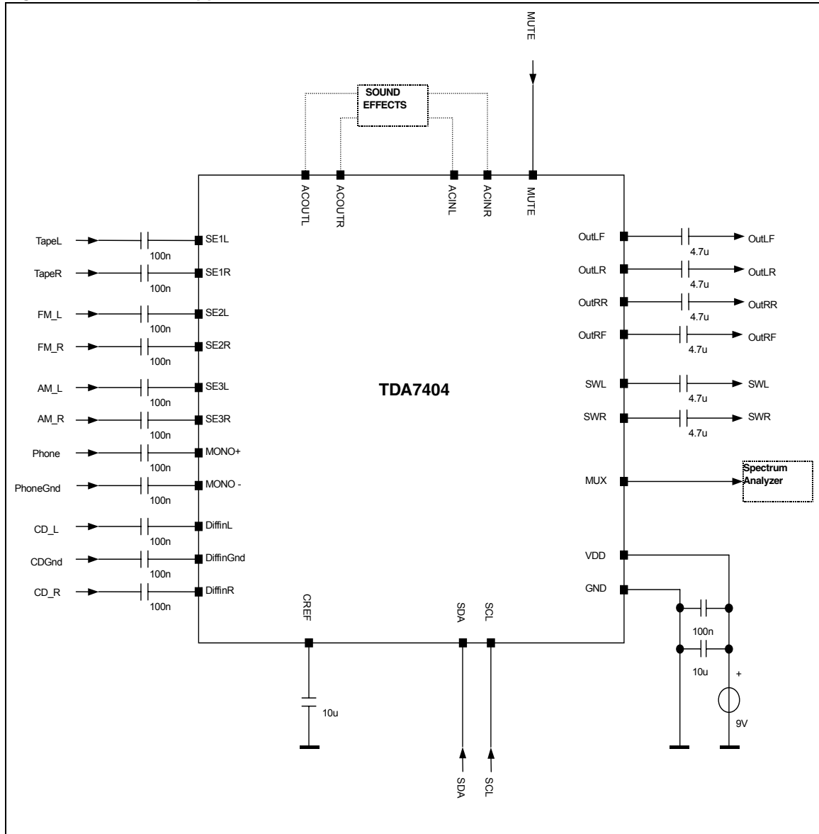
Figure 18. TDA7404 application circuit
