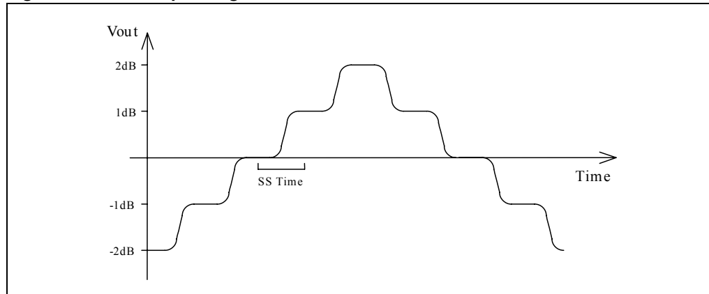
Figure 9. Soft-step timing
