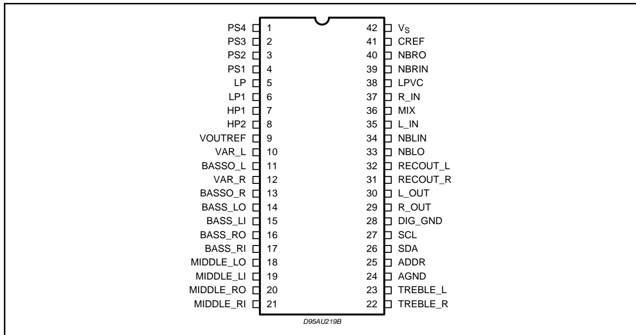
Figure 3. Pin Connection (TDA7431)
