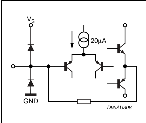
Figure 23. PIN: ADDR
