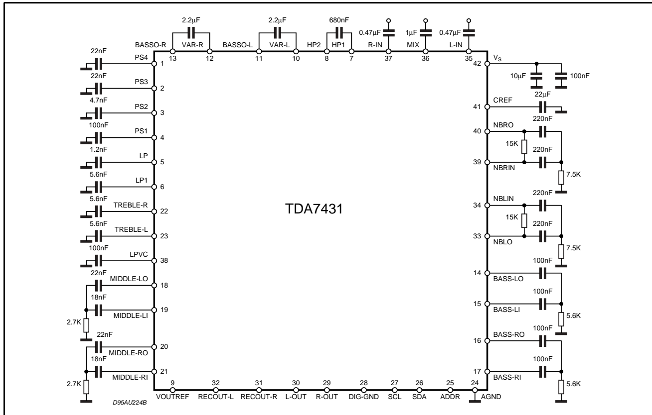
Figure 5. TEST CIRCUIT (TDA7431)
