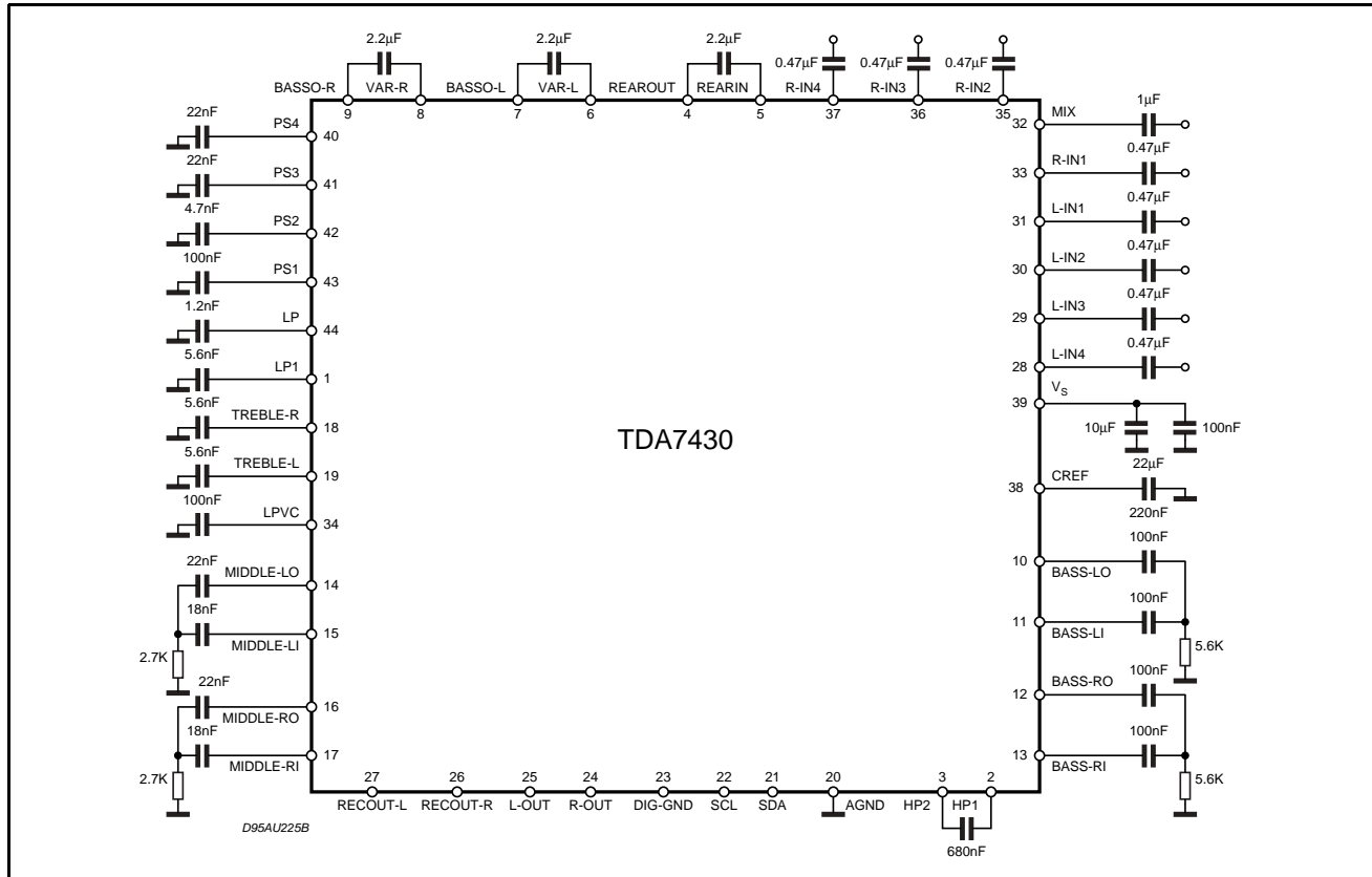
Figure 4. TEST CIRCUIT (TDA7430)
