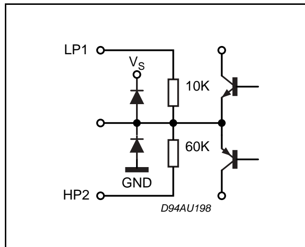
Figure 15. PIN: HP1
