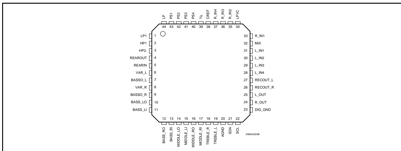
Figure 2. Pin Connection (TDA7430)
