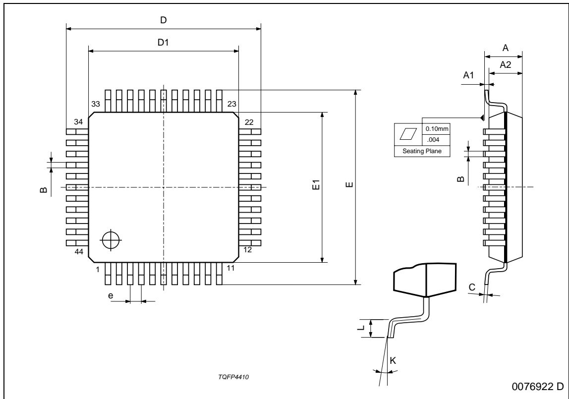
TQFP44 (10 x 10 x 1.4mm)
