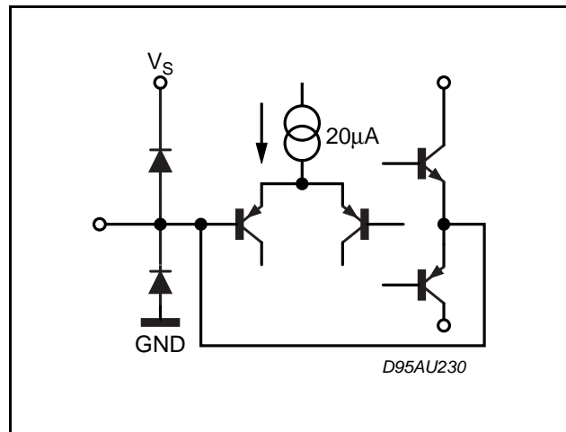
Figure 27. BASS-LI, BASS-RI, MIDDLE-L, MIDDLE-RII
