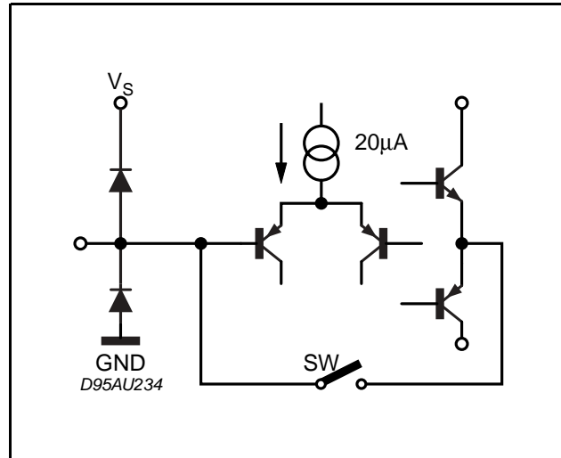
Figure 32. NBLO, NBRO
