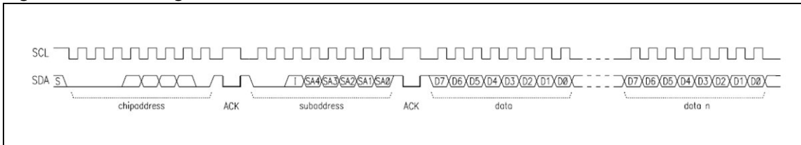
Figure 21. Switching characteristics
