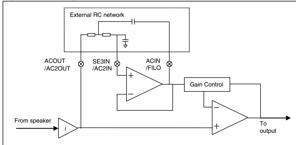
Figure 22. HPF diagram
