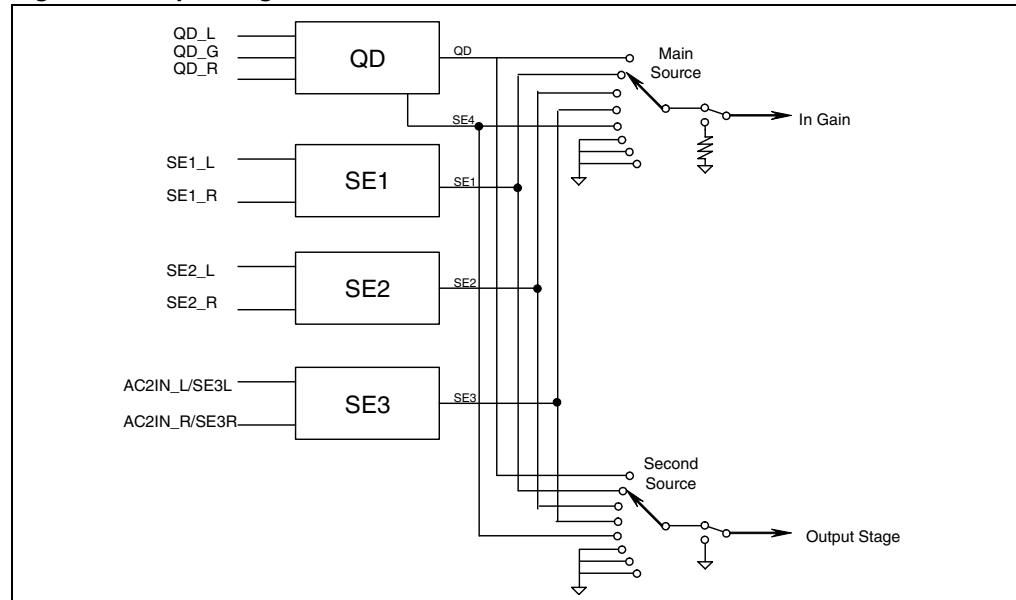
Figure 3. Input stage
