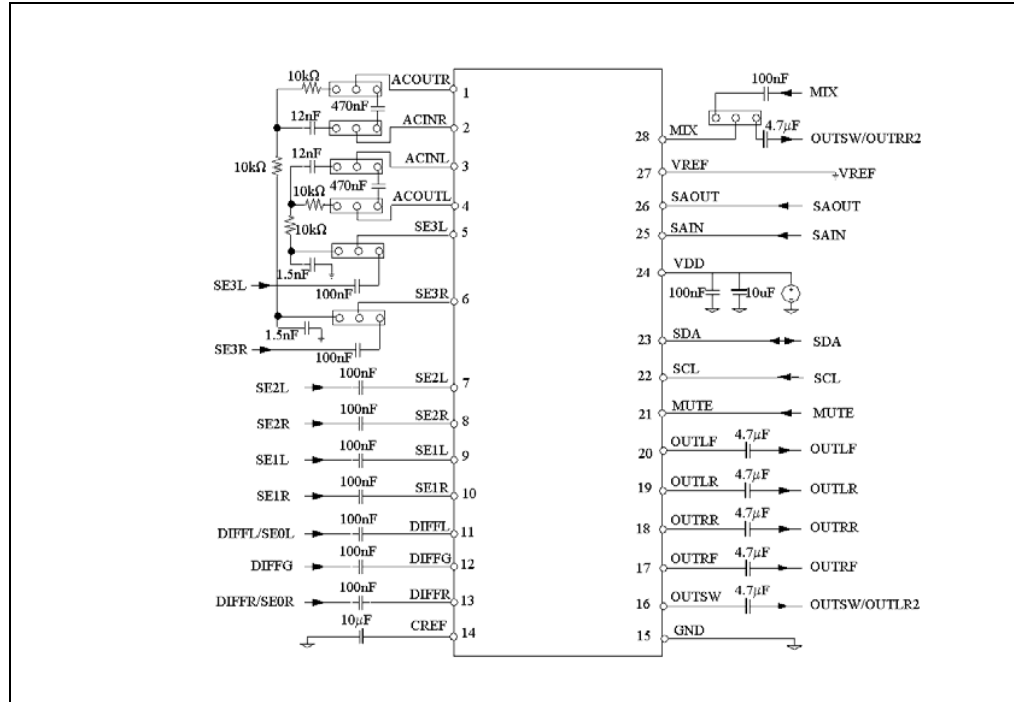
Figure 24. Test circuit
