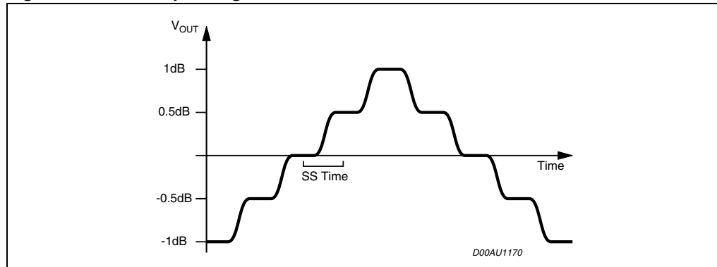
Figure 8. Soft-step timing
