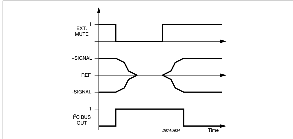
Figure 7. Soft-mute timing
