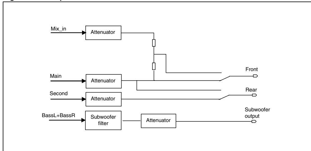
Figure 23. Output selector
