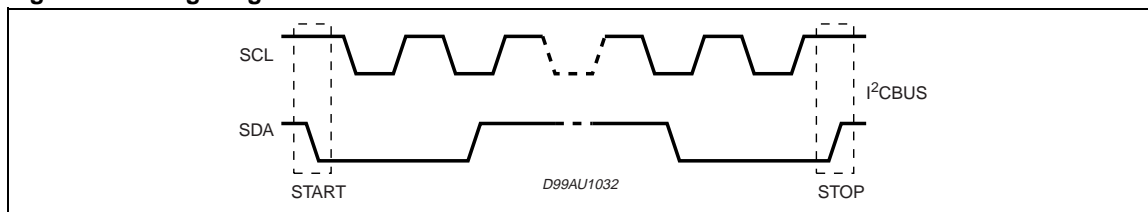
Figure 3. Timing Diagram on the I 2 C BUS
