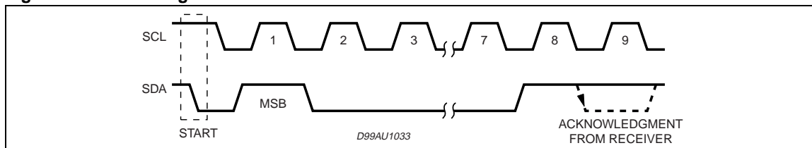
Figure 4. Acknowledge on the I 2 C BUS
