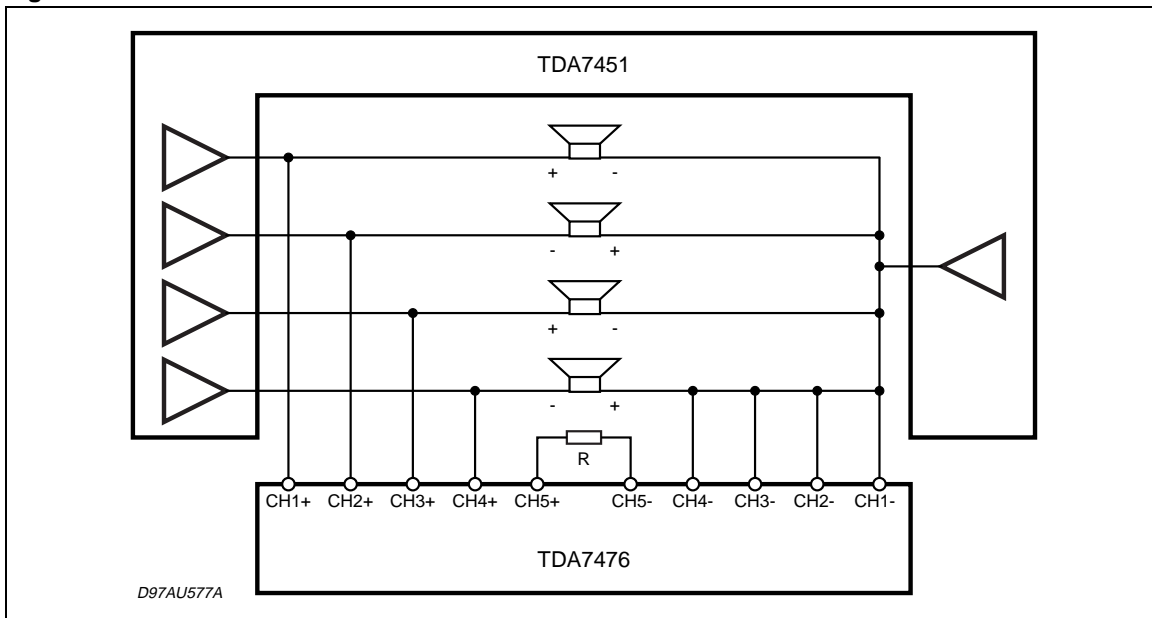
Figure 6. TDA7451
