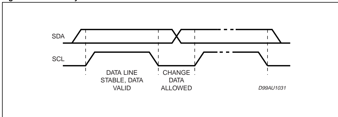
Figure 2. Data Validity on the I 2 C BUS
