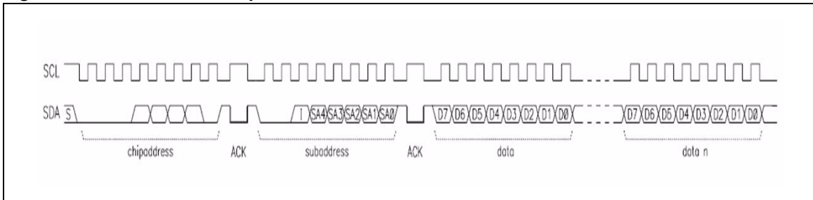
Figure 20. I 2 C bus interface protocol
