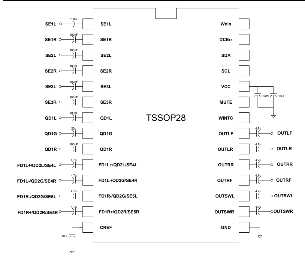
Figure 19. Test circuit
