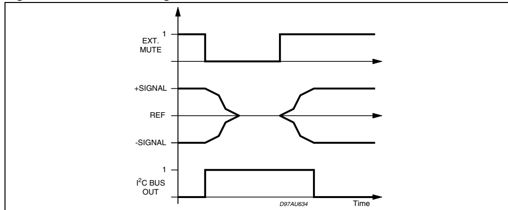
Figure 7. SoftMute timing
