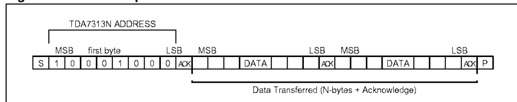
Figure 23. Interface protocol
