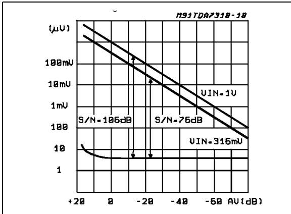
Figure 8. Signal to noise ratio vs. volume setting
