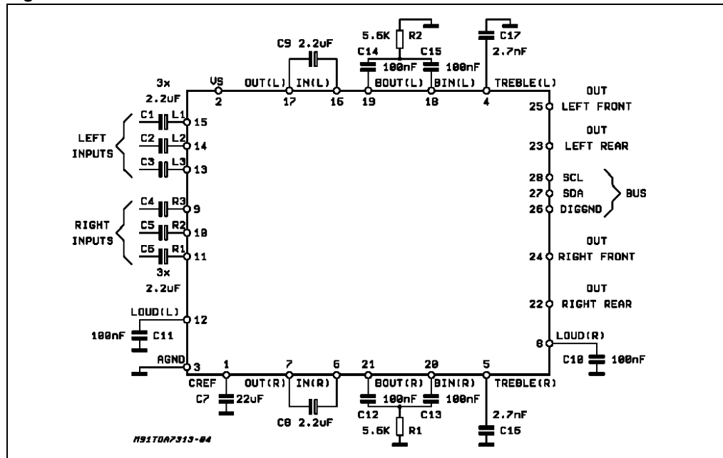
Figure 2. Test circuit
