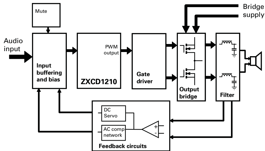
ZXCDSUBEV series architecture
