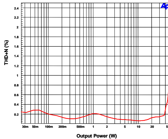
ZXCD50STEVAL THD+N versus output power
