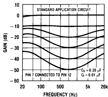
FIGURE 7. Loudness Compensated Volume Characteristic
