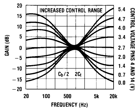
FIGURE 2. Tone Characteristic (Gain vs Frequency)
