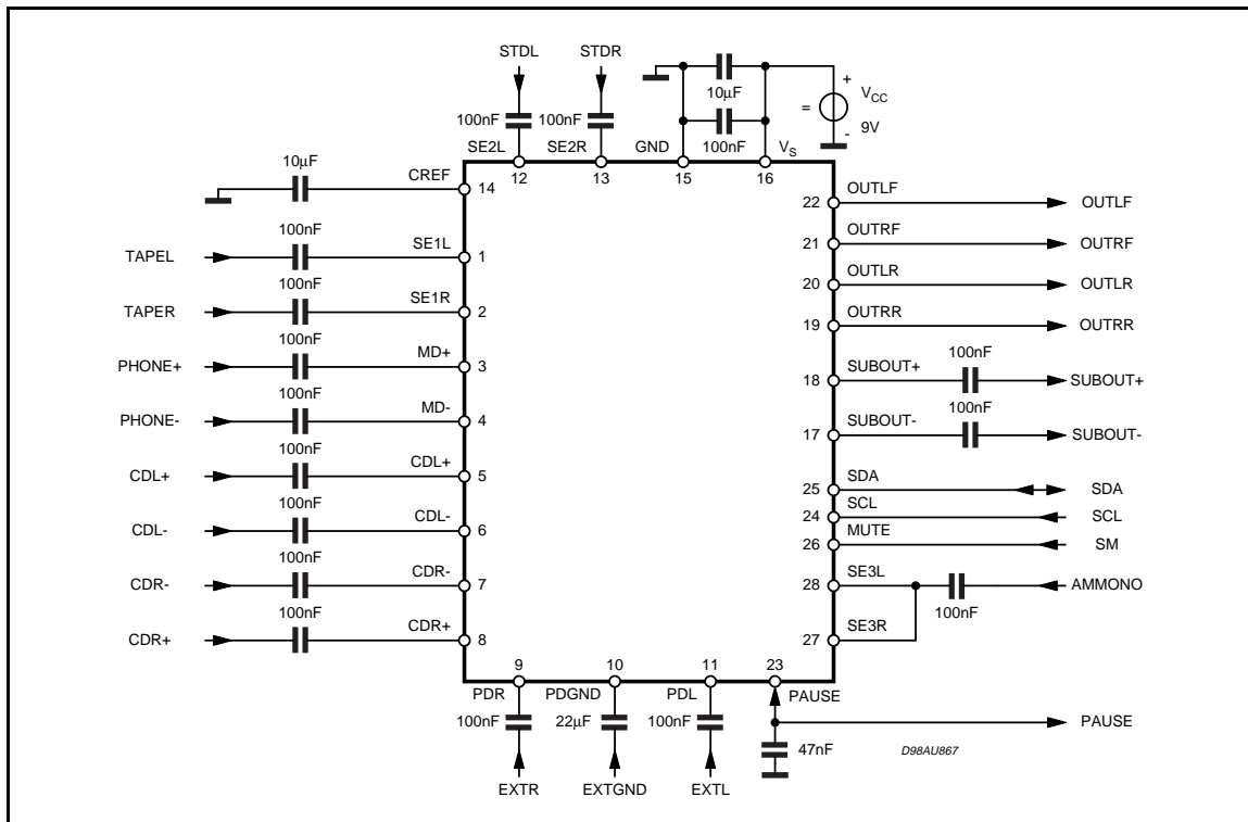
Figure 18. Application Circuit.
