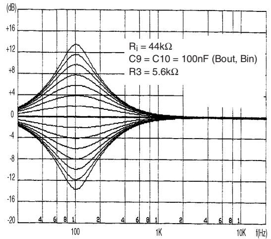
Figure 9. Bass response
