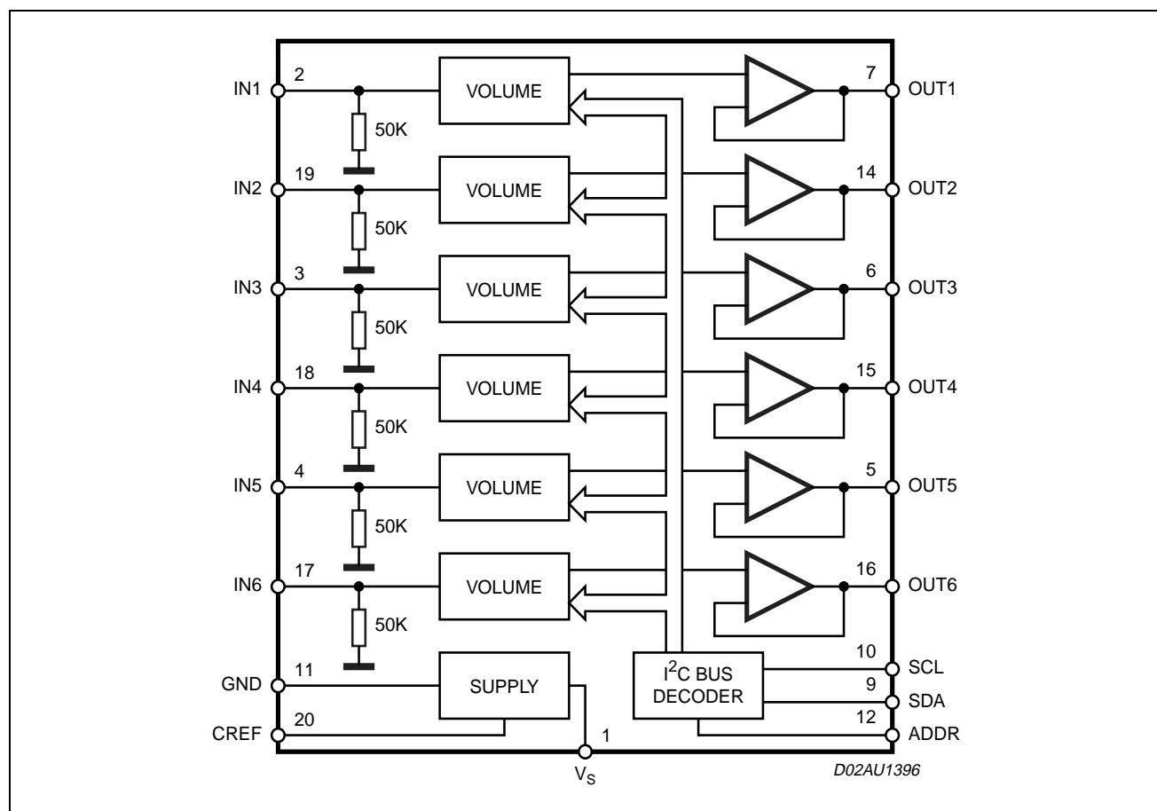
Figure 2. Block Diagram
