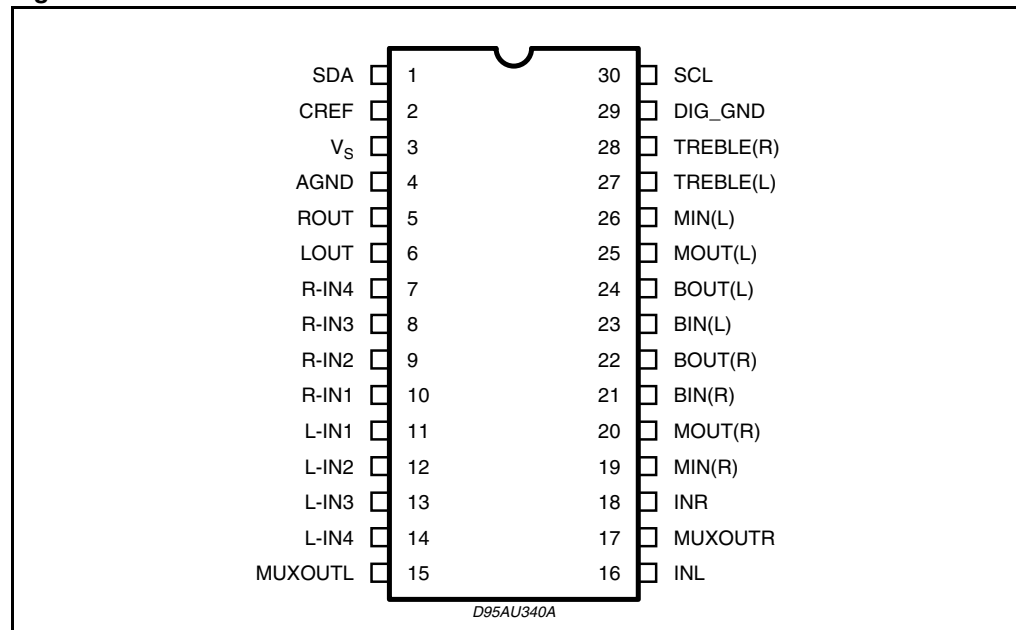
Figure 2. Pin connections
