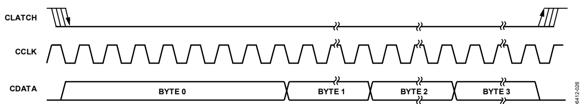
Figure 26. SPI Write to ADAU1701 Clocking (Single-Write Mode)
