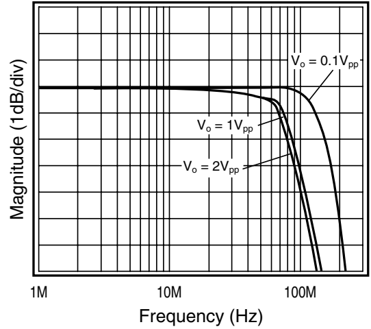
Frequency Response vs. V_o
