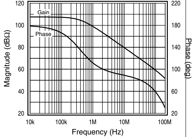
Open Loop Transimpedance Gain, Z(s)
