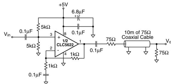
FIGURE 10. Single Supply Cable Driver
