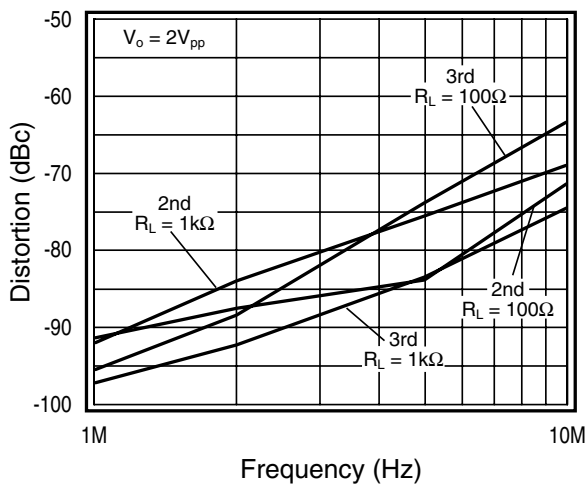
2nd & 3rd Harmonic Distortion
