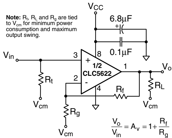
FIGURE 1. Non-Inverting Configuration
