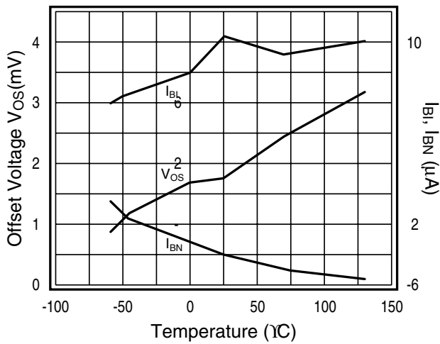
I_{BI} , I_{BN} , V_{OS} vs. Temperature
