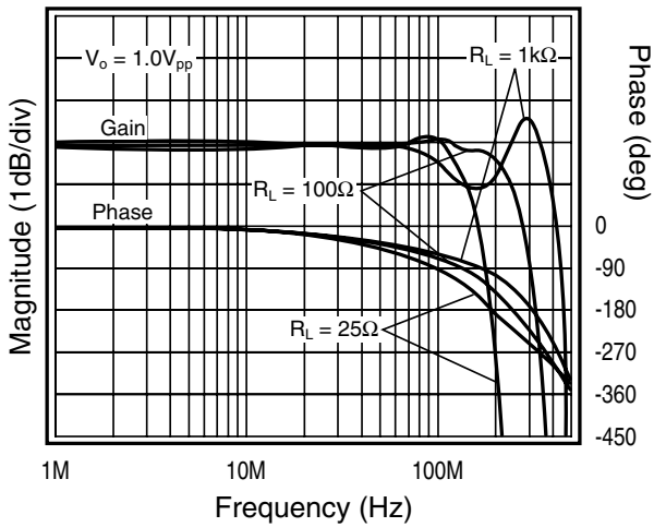
Frequency Response vs. R_L
