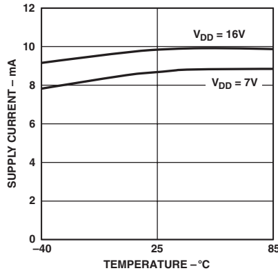
TPC 14. Supply Current vs. Temperature
