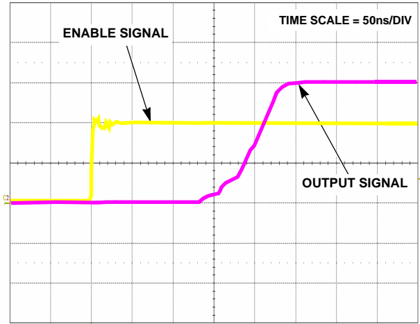
FIGURE 13. ENABLE TIME
