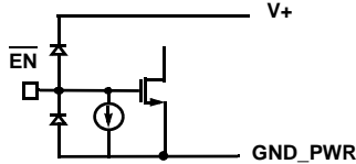
CIRCUIT 2
