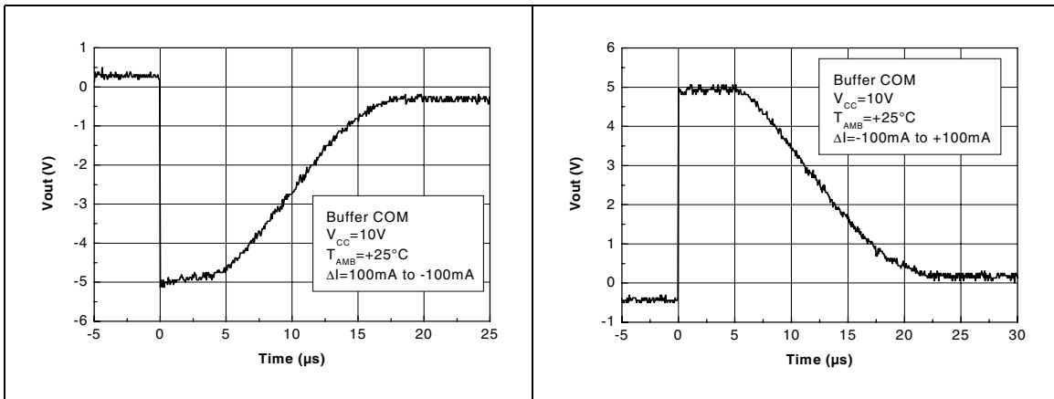
Figure 42. Output voltage response to current transient - buffer COM Figure 43. Output voltage response to current transient - buffer COM
