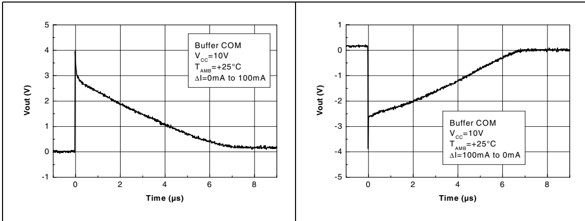
Figure 40. Output voltage response to current transient - buffer COM Figure 41. Output voltage response to current transient - buffer COM
