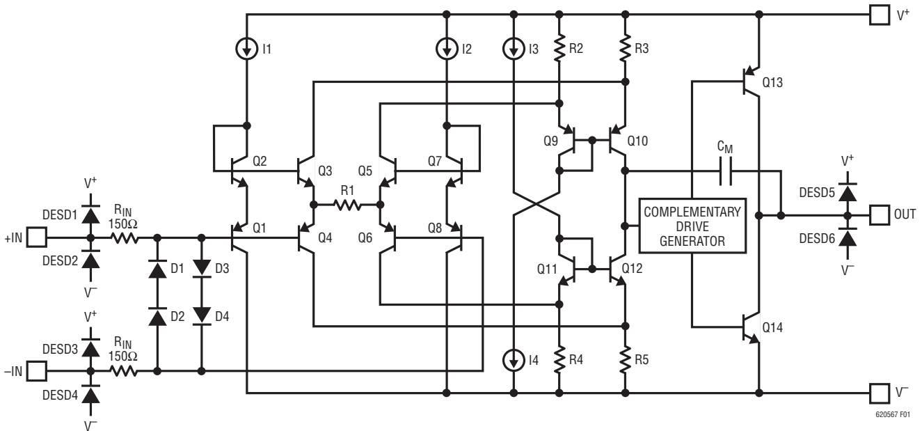
Figure 1. Simplified Schematic
