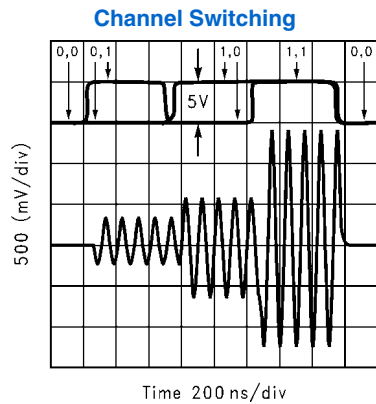
FIGURE 7. PGA Output
