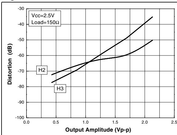
Figure 5. Distortion at Vcc=2.5 V
