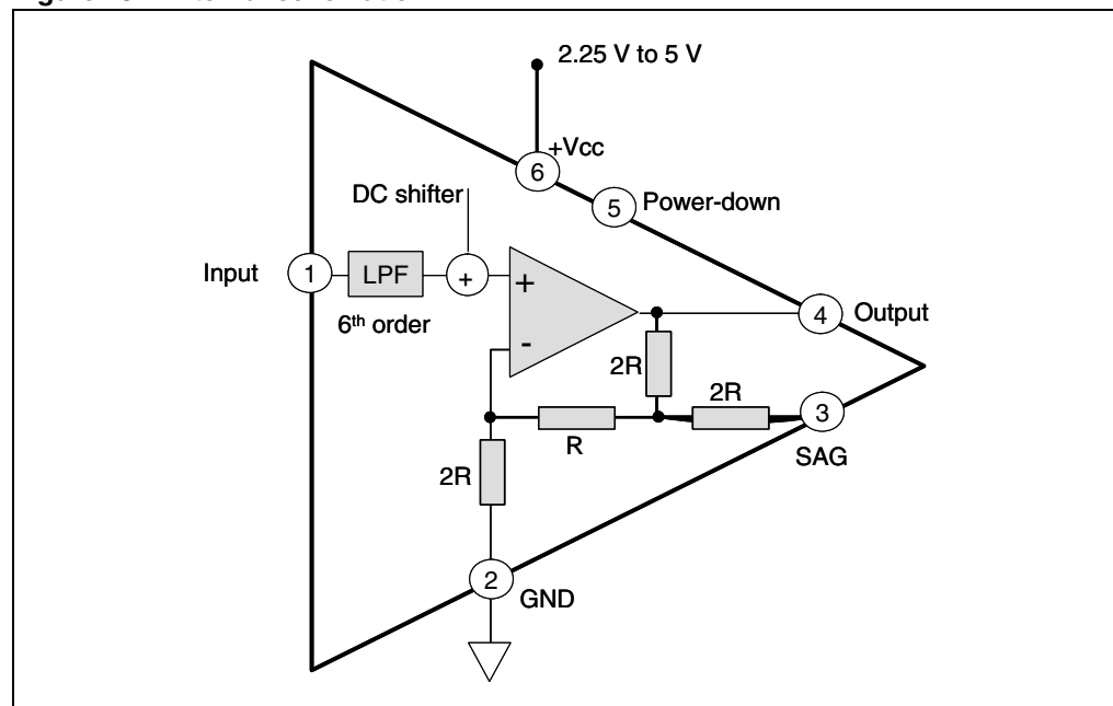
Figure 25. Internal schematic
