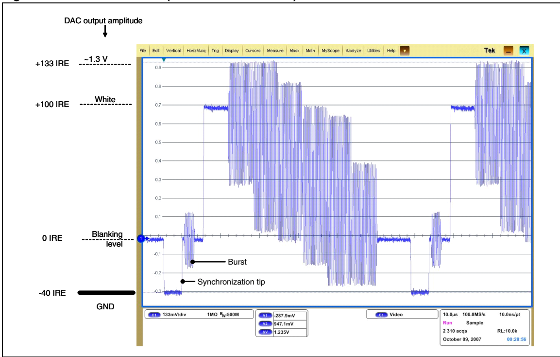
Figure 28. Details on Cvbs (NTSC color bar 100%)
