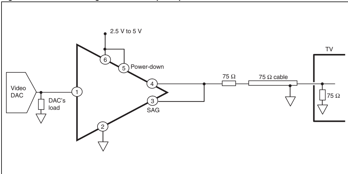
Figure 27. Schematic diagram without output capacitor
